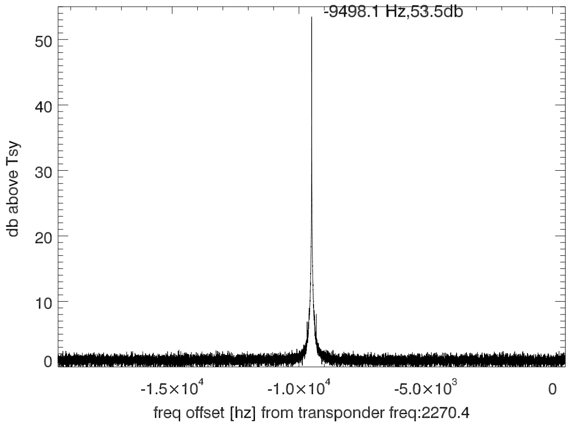
isee3 140609:195105 (UTC) spectra after doppler correction. PolB
