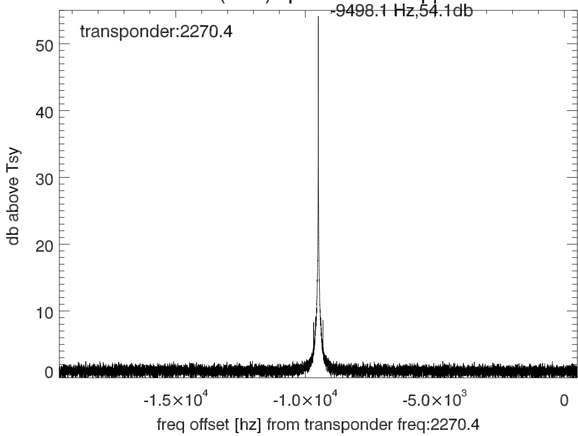
isee3 140609:195105 (UTC) spectra after doppler correction. PolA
