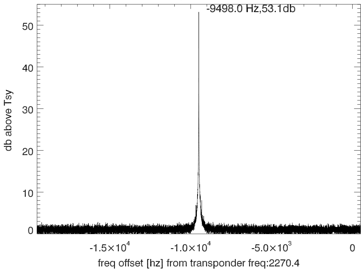
isee3 140609:194621 (UTC) spectra after doppler correction. PolB
