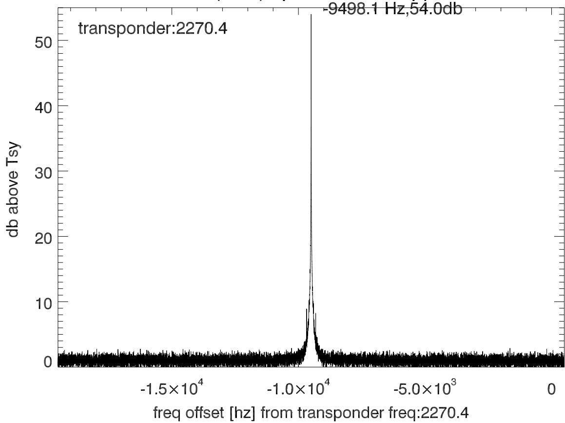
isee3 140609:194621 (UTC) spectra after doppler correction. PolA
