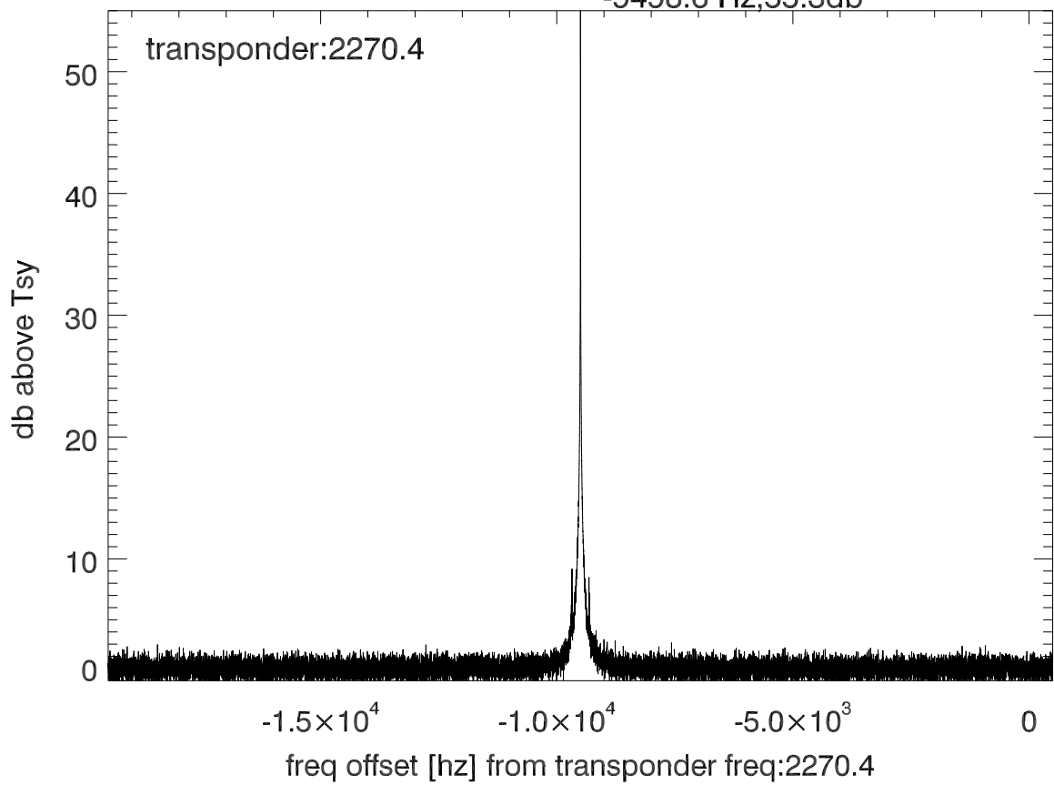
isee3 140609:193239 (UTC) spectra after doppler correction. PolA
