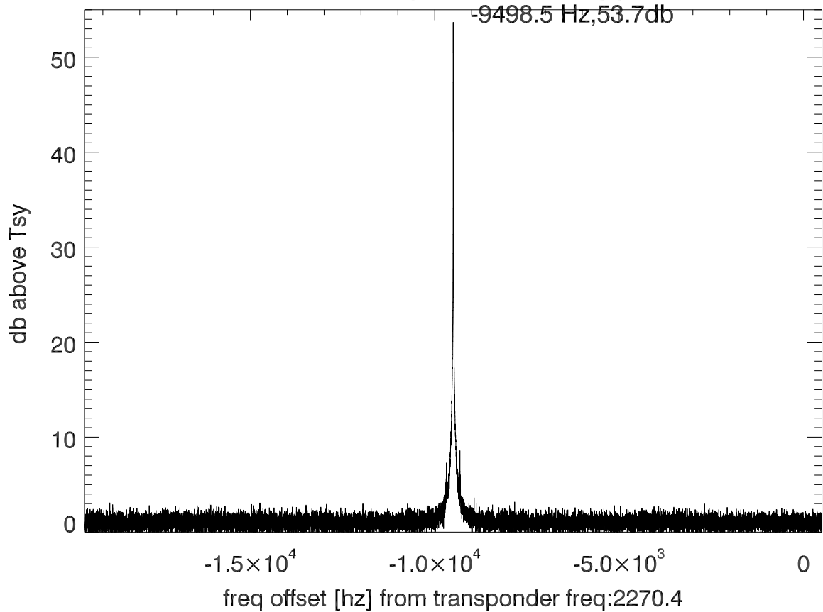
isee3 140609:193239 (UTC) spectra after doppler correction. PolB
