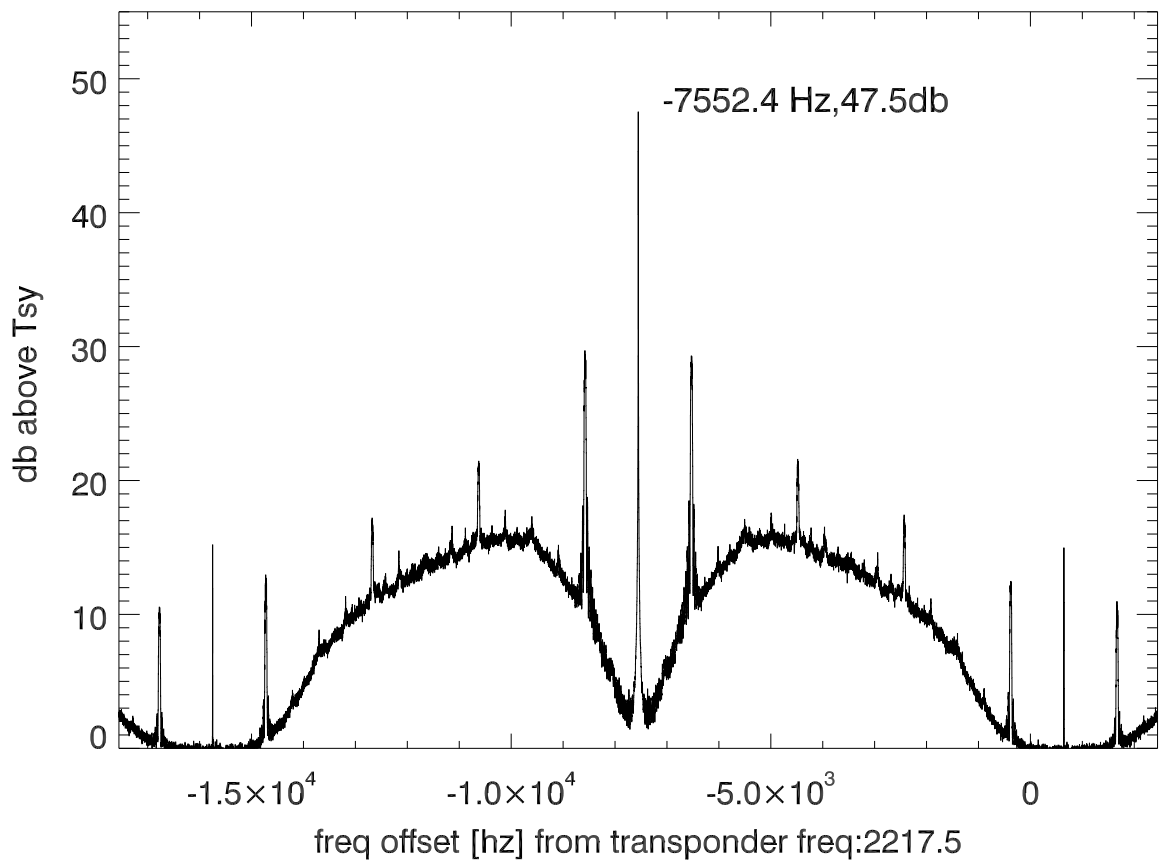
isee3 140609:201412 (UTC) spectra after doppler correction. PoIB
