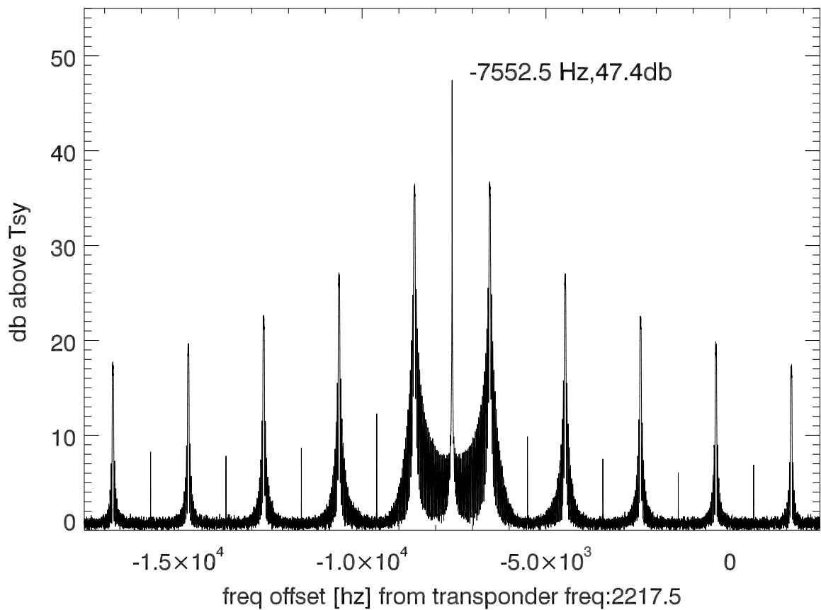
isee3 140609:200730 (UTC) spectra after doppler correction. PolB
