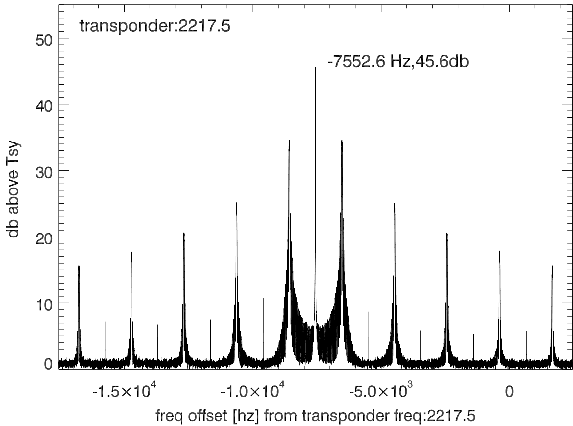
isee3 140609:200730 (UTC) spectra after doppler correction. PolA
