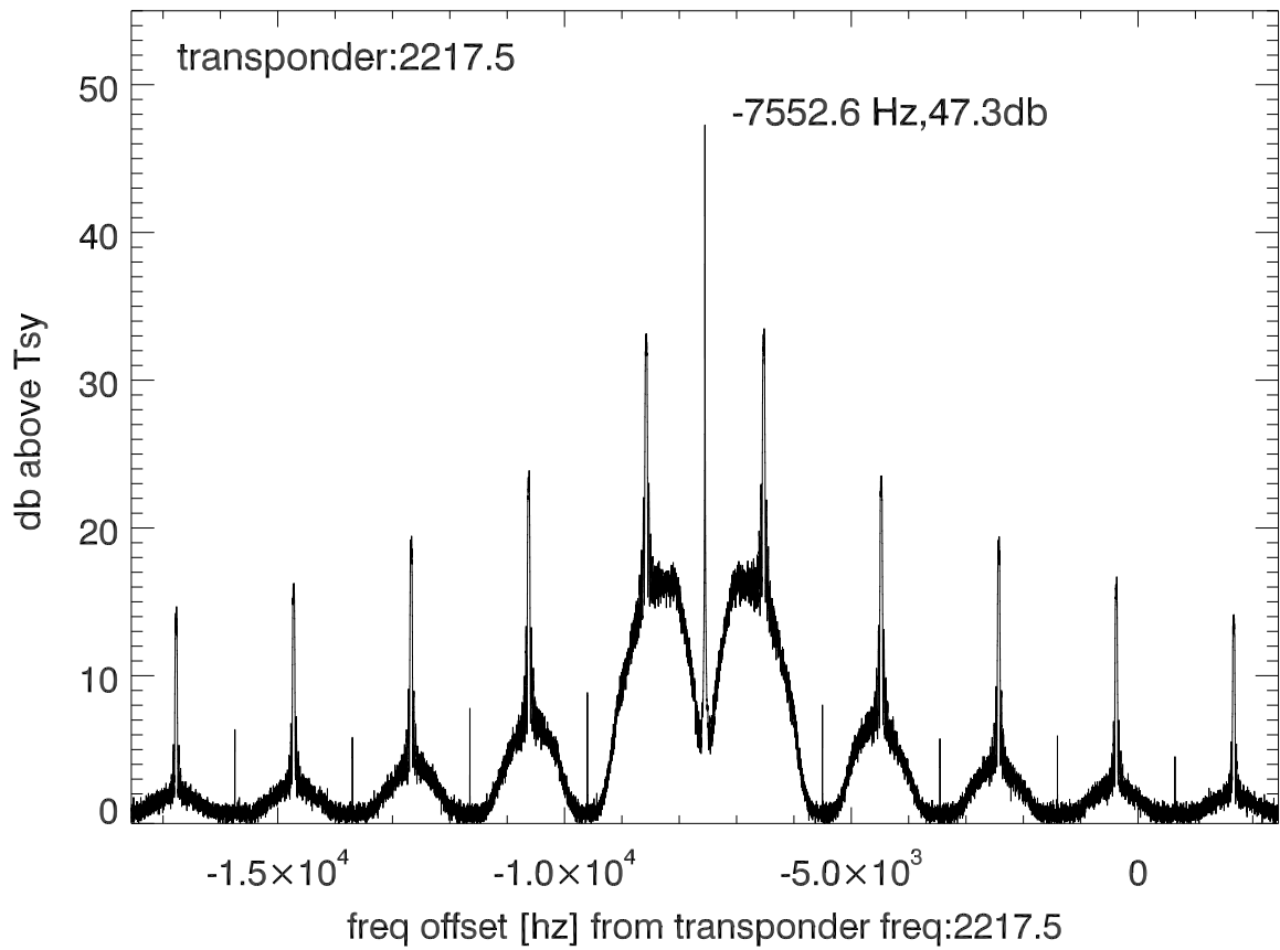
isee3 140609:200401 (UTC) spectra after doppler correction. PoIA
