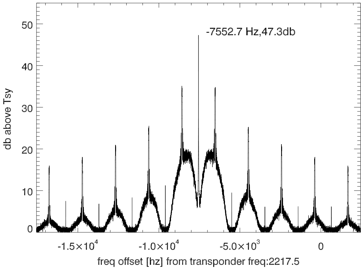
isee3 140609:200020 (UTC) spectra after doppler correction. PoIB
