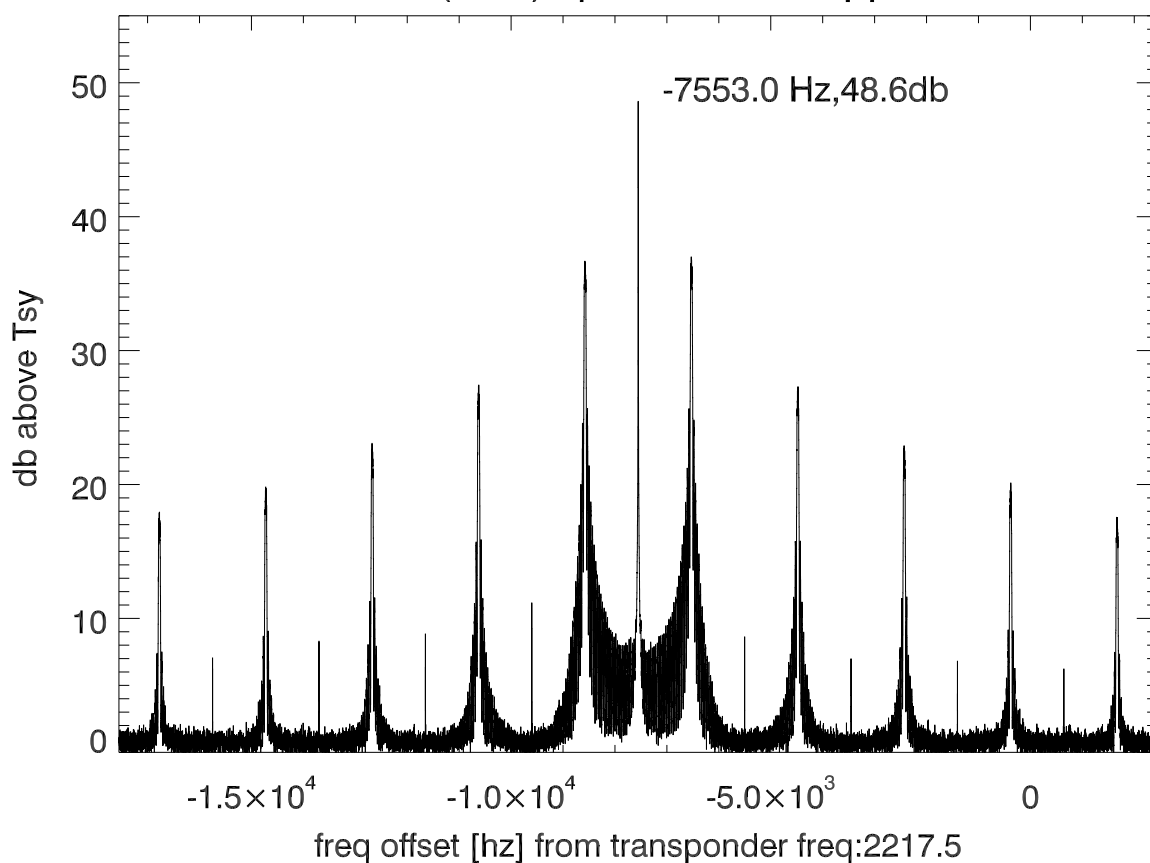
isee3 140609:195105 (UTC) spectra after doppler correction. PoIB
