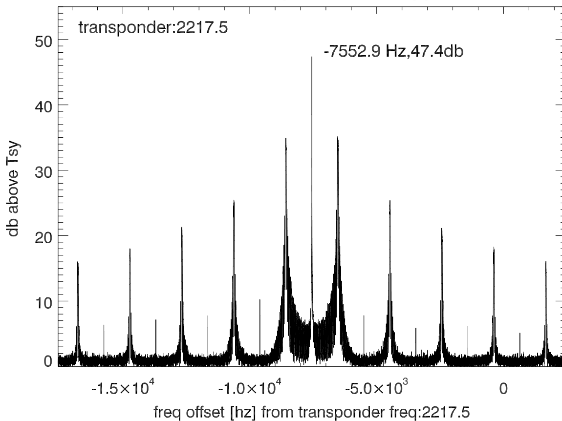
isee3 140609:195105 (UTC) spectra after doppler correction. PoIA
