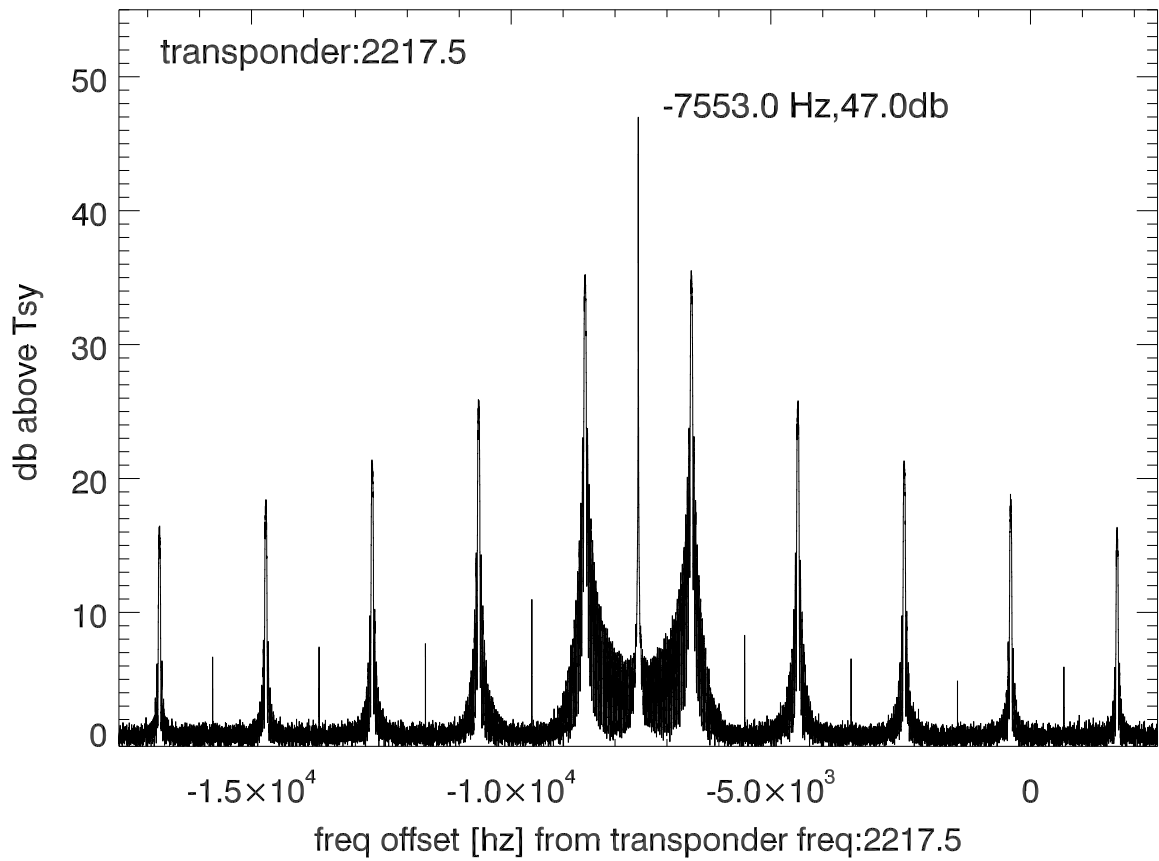
isee3 140609:194824 (UTC) spectra after doppler correction. PolA
