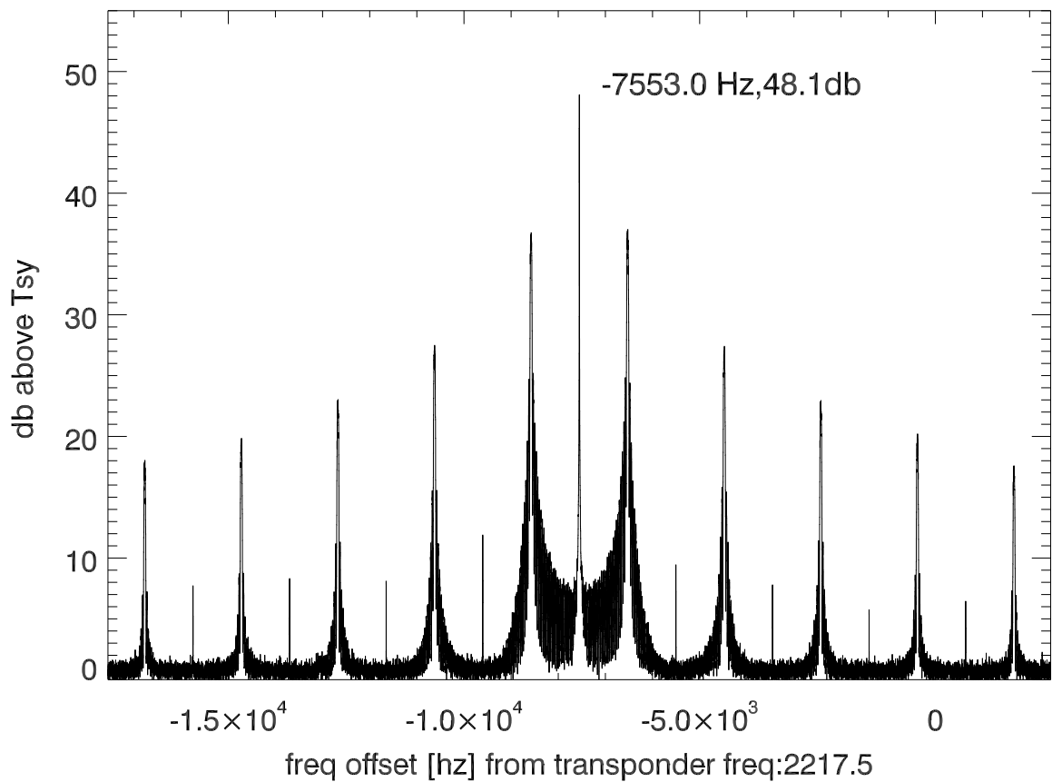
isee3 140609:194824 (UTC) spectra after doppler correction. PolB
