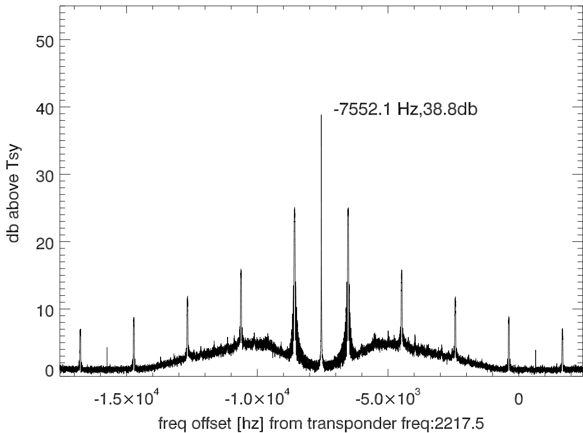
isee3 140609:204346 (UTC) spectra after doppler correction. PoIB
