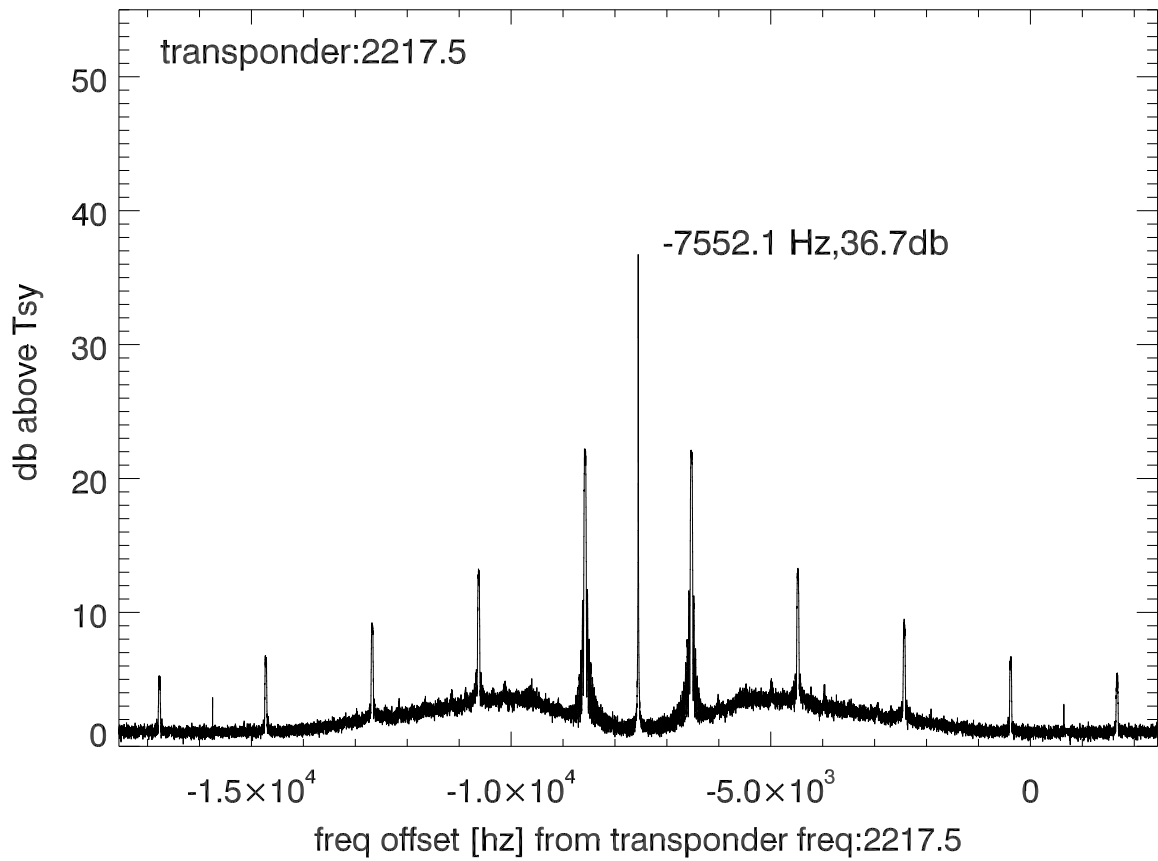
isee3 140609:204346 (UTC) spectra after doppler correction. PoIA
