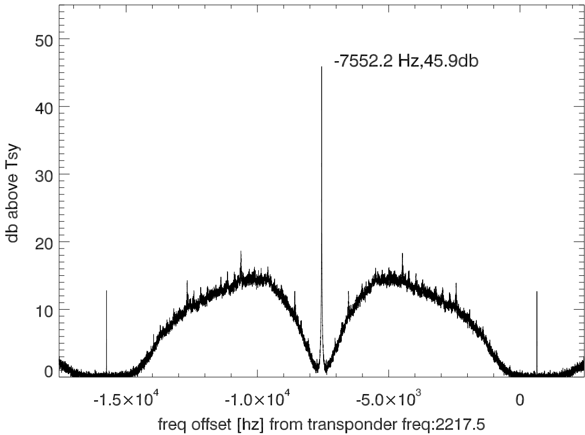
isee3 140609:203516 (UTC) spectra after doppler correction. PoIB
