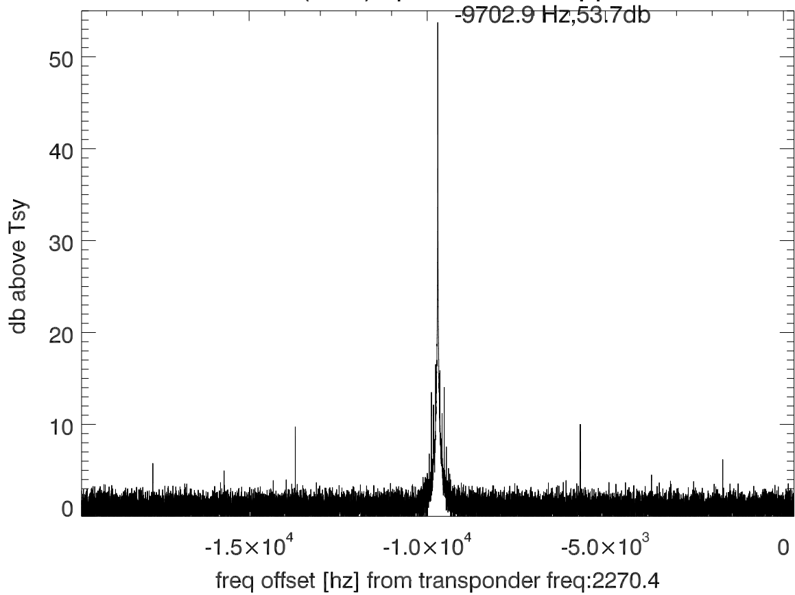
isee3 140606:202243 (UTC) spectra after doppler correction. PolB
