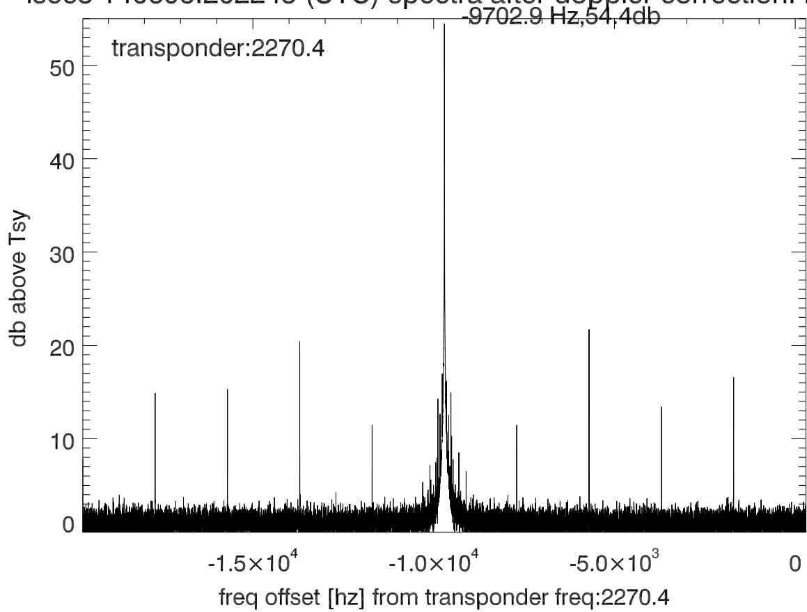
isee3 140606:202243 (UTC) spectra after doppler correction. PolA
