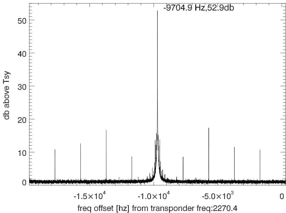
isee3 140606:195158 (UTC) spectra after doppler correction. PolB
