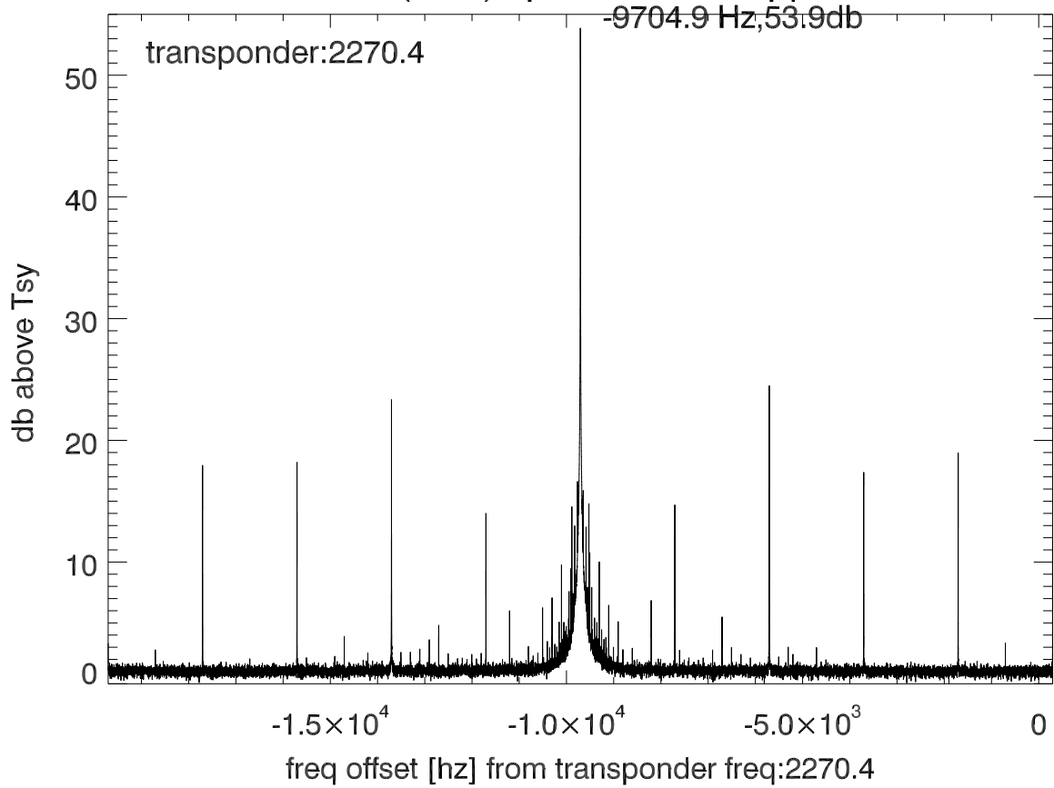
isee3 140606:195158 (UTC) spectra after doppler correction. PolA
