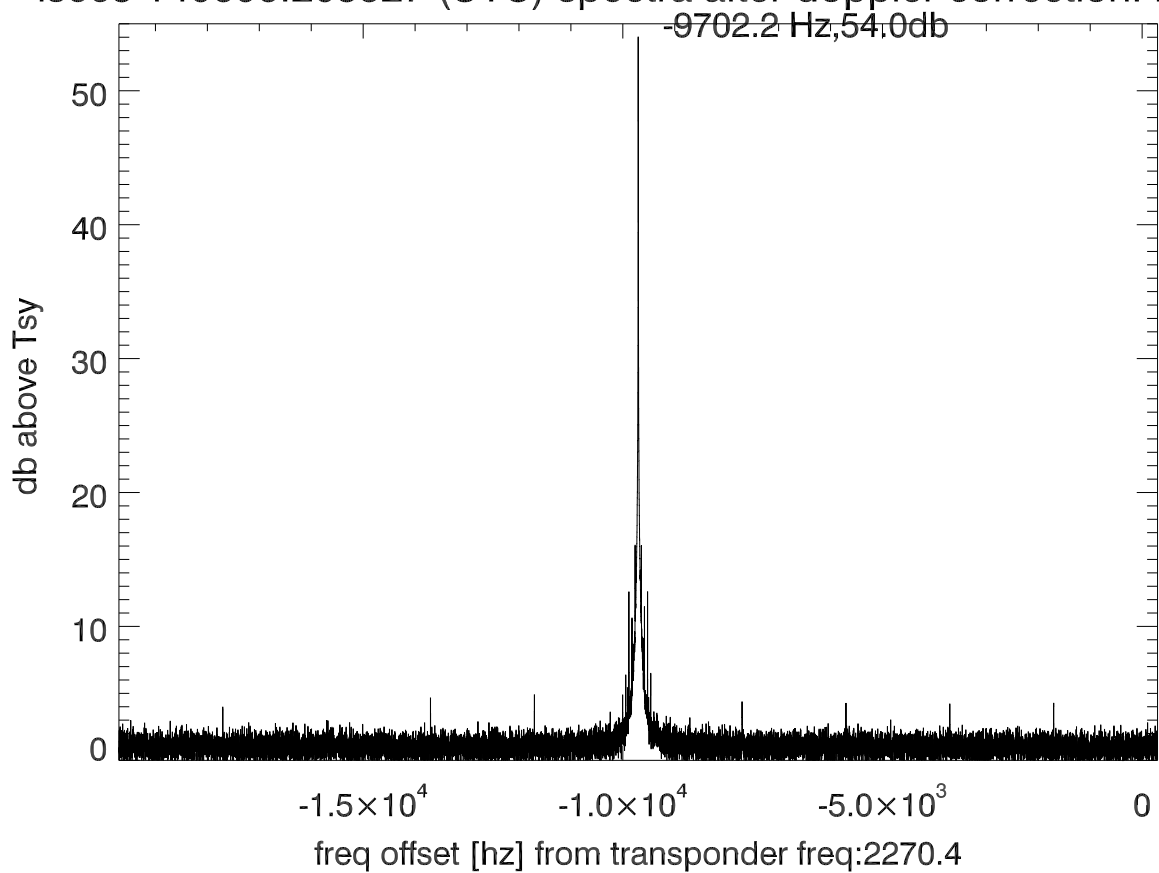
isee3 140606:203527 (UTC) spectra after doppler correction. PolB
