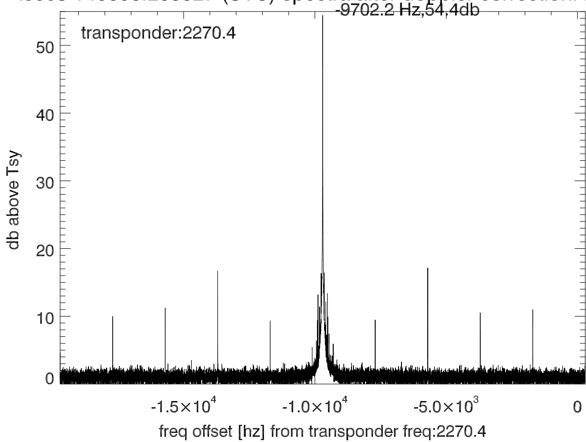
isee3 140606:203527 (UTC) spectra after doppler correction. PolA
