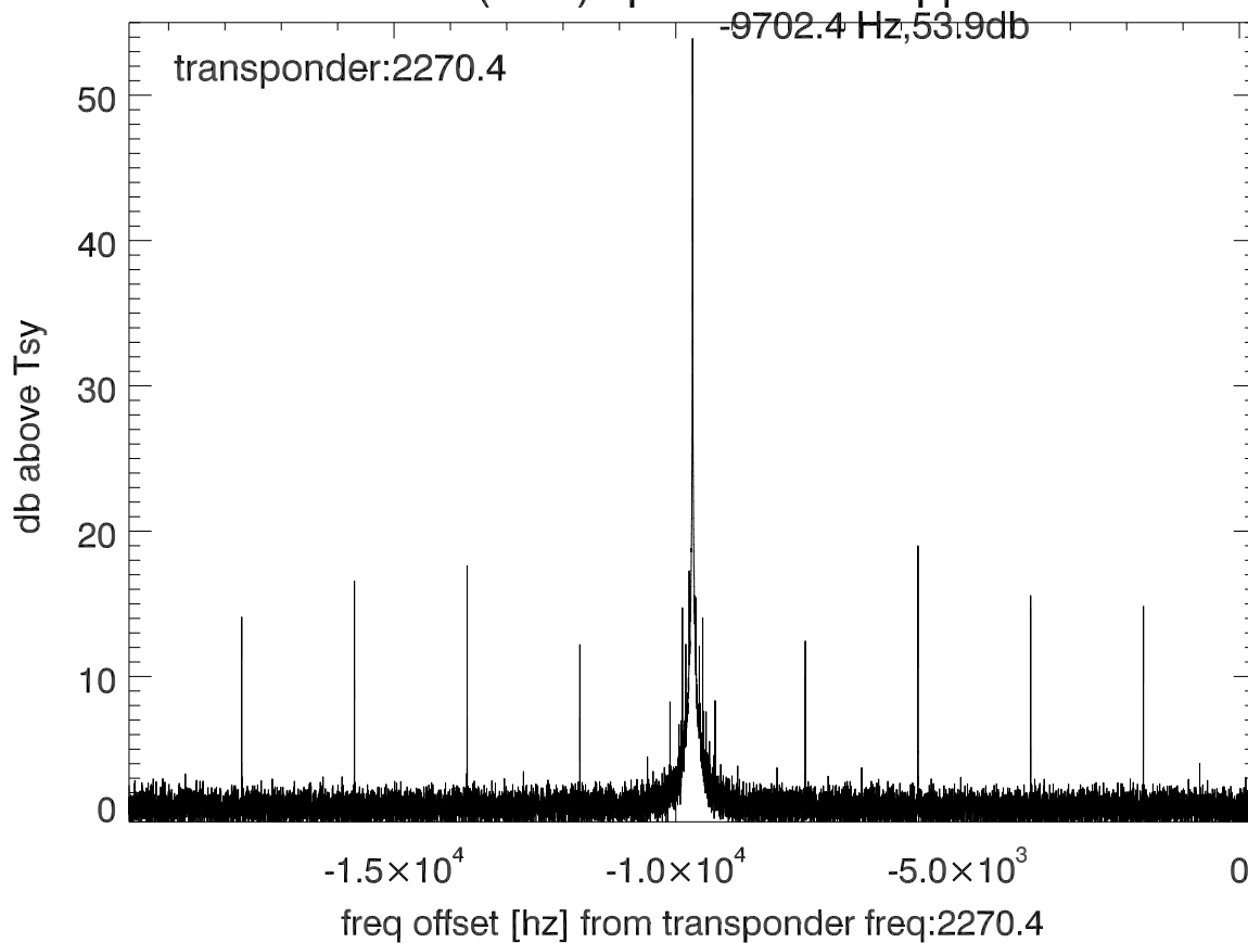
isee3 140606:203153 (UTC) spectra after doppler correction. PolA
