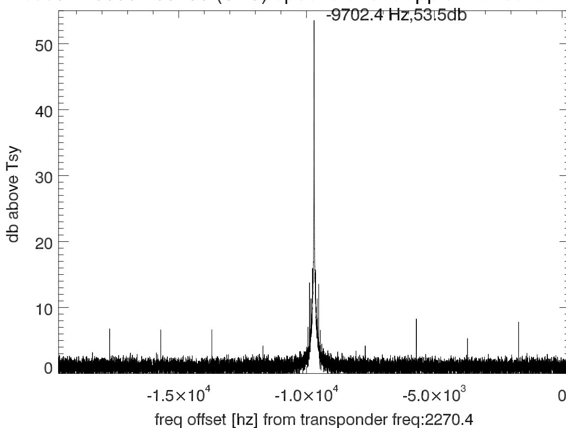
isee3 140606:203153 (UTC) spectra after doppler correction. PolB
