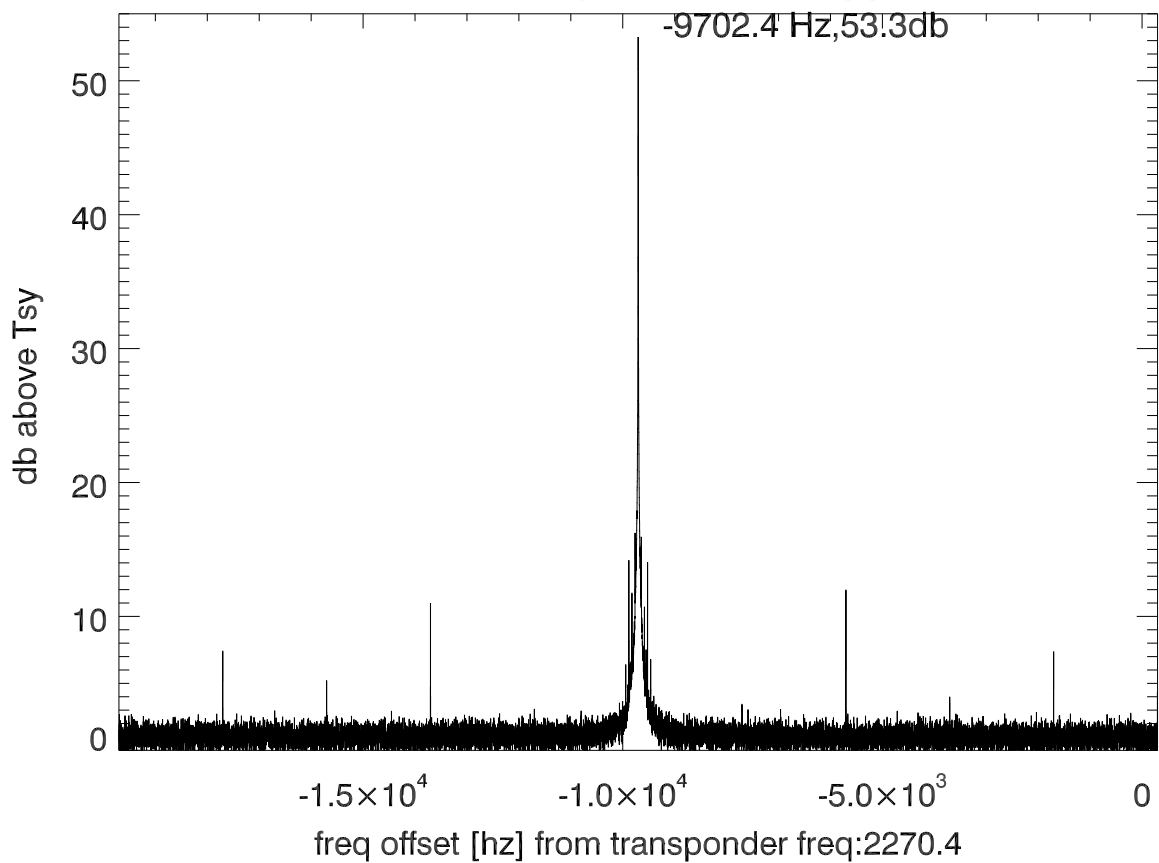
isee3 140606:202819 (UTC) spectra after doppler correction. PolB
