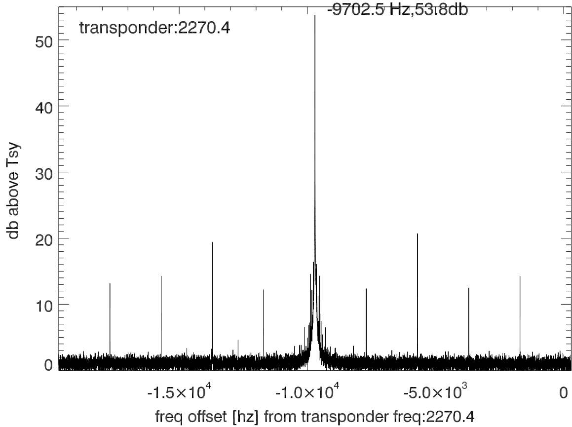
isee3 140606:202819 (UTC) spectra after doppler correction. PolA
