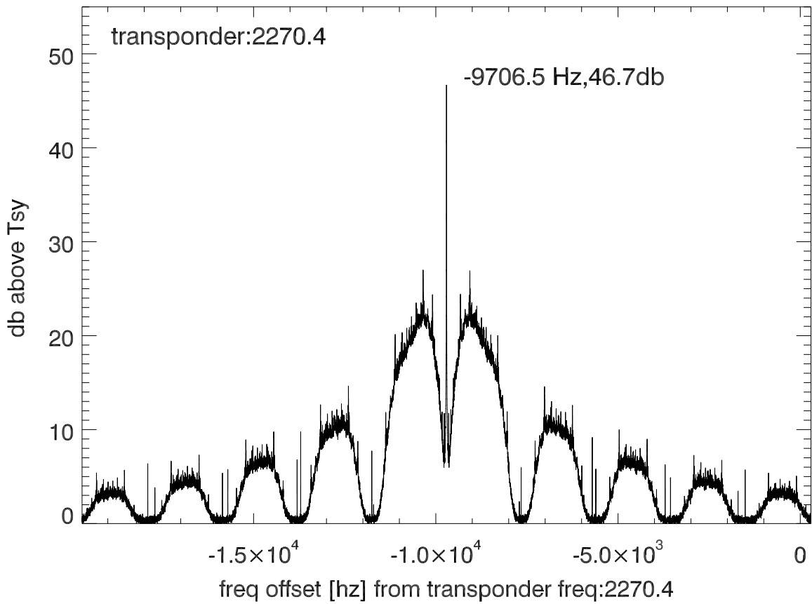
isee3 140606:190955 (UTC) spectra after doppler correction. PolA
