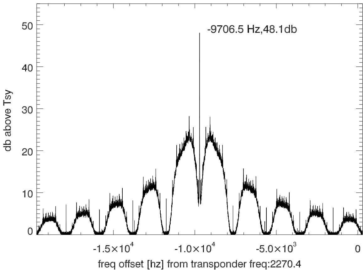
isee3 140606:190955 (UTC) spectra after doppler correction. PolB
