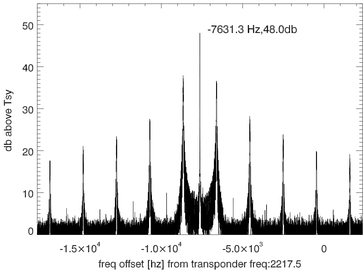
isee3 140606:202042 (UTC) spectra after doppler correction. PolB
