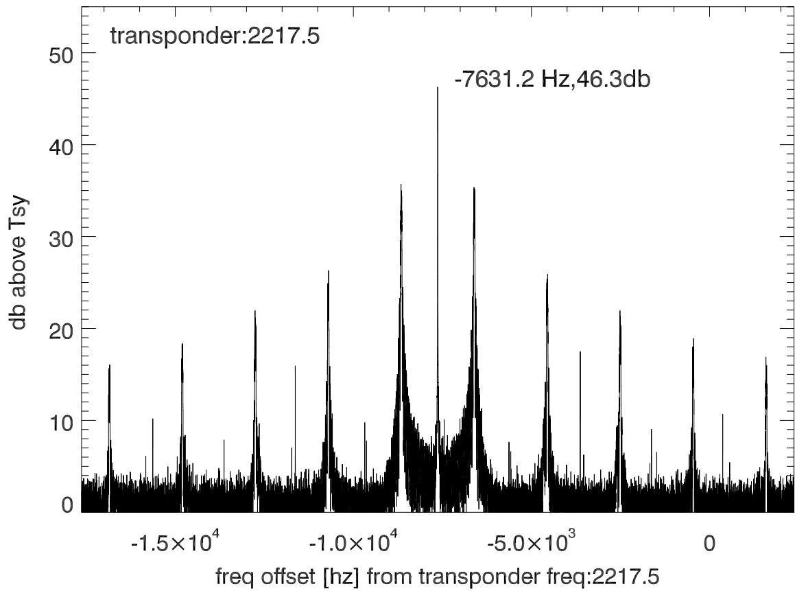
isee3 140606:202042 (UTC) spectra after doppler correction. PolA
