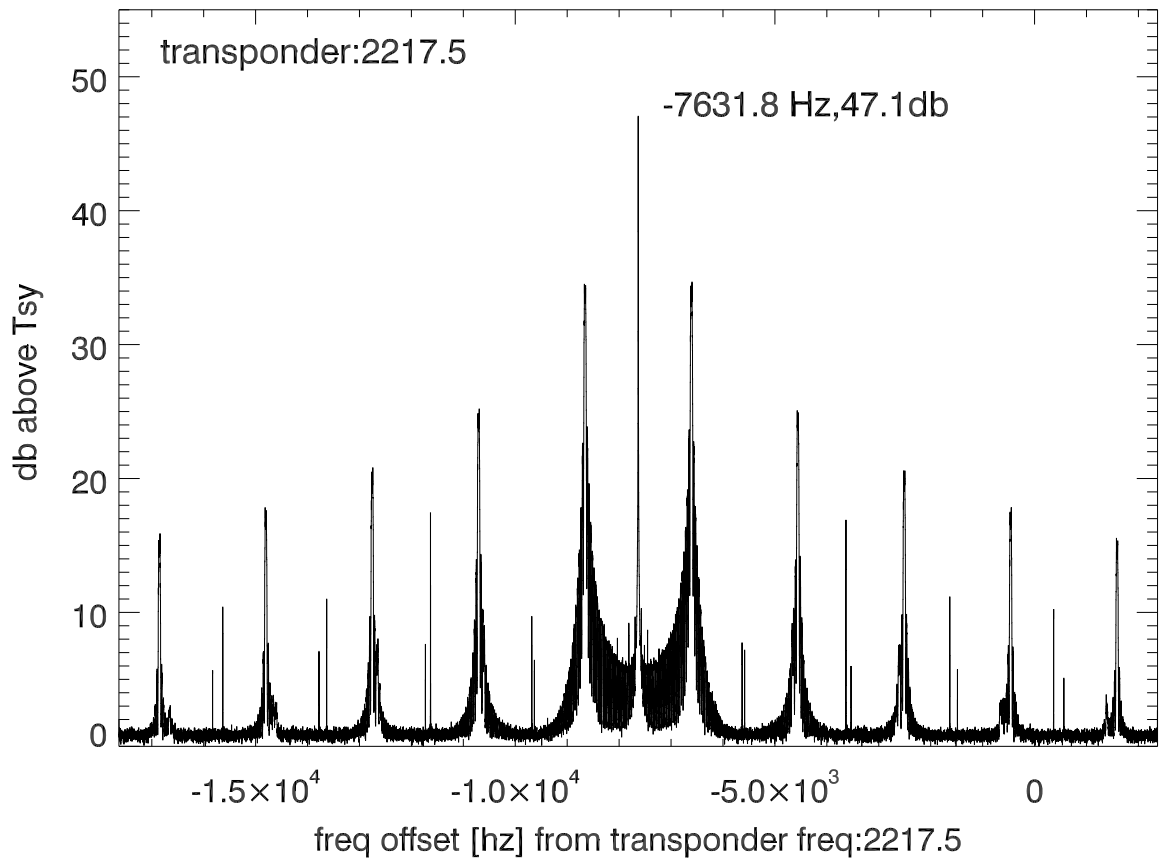
isee3 140606:195158 (UTC) spectra after doppler correction. PoIA
