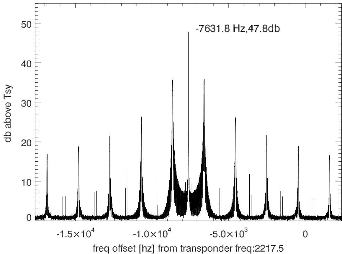
isee3 140606:195158 (UTC) spectra after doppler correction. PoIB
