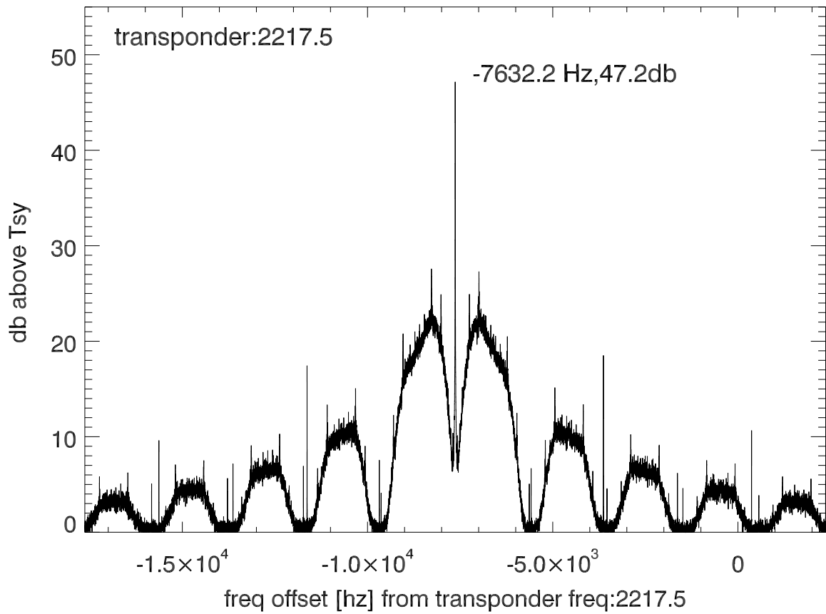
isee3 140606:193106 (UTC) spectra after doppler correction. PoIA
