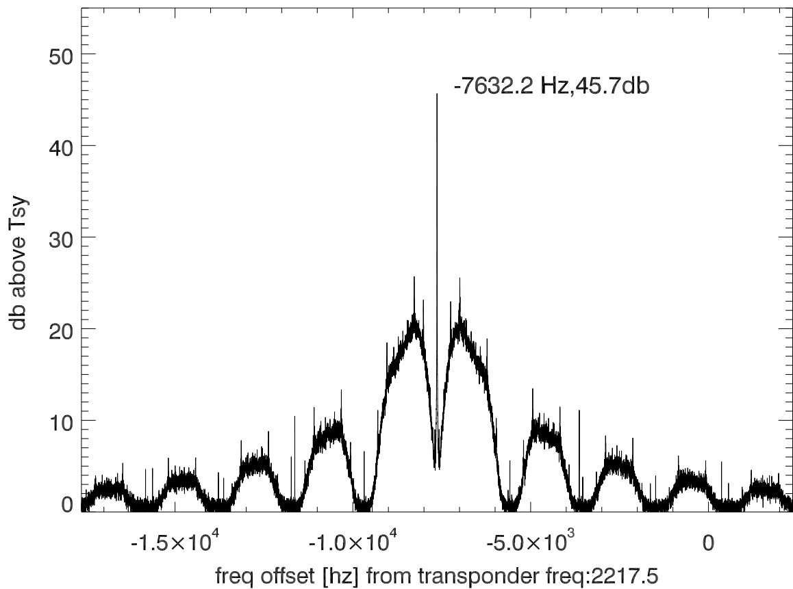
isee3 140606:193106 (UTC) spectra after doppler correction. PoIB
