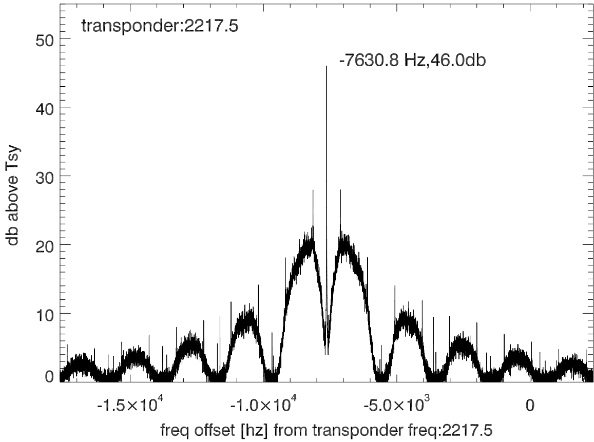
isee3 140606:203527 (UTC) spectra after doppler correction. PoIA
