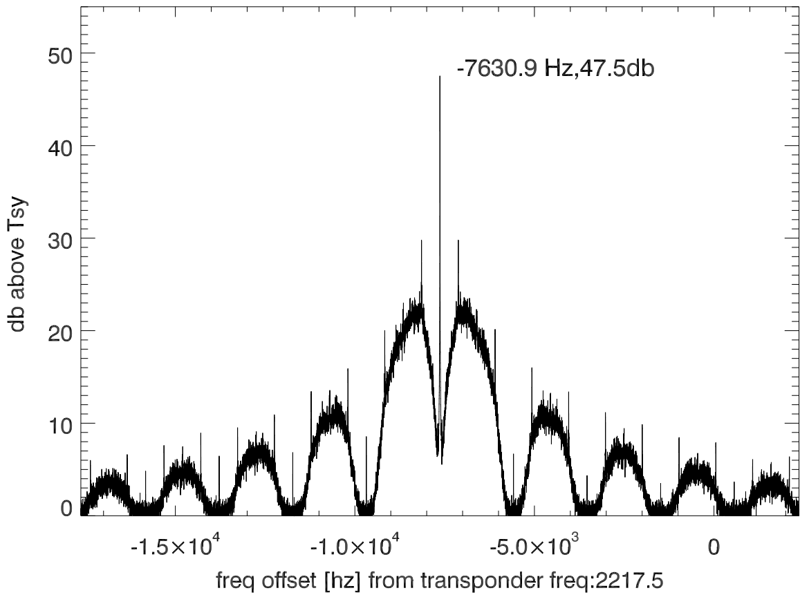
isee3 140606:203527 (UTC) spectra after doppler correction. PoIB
