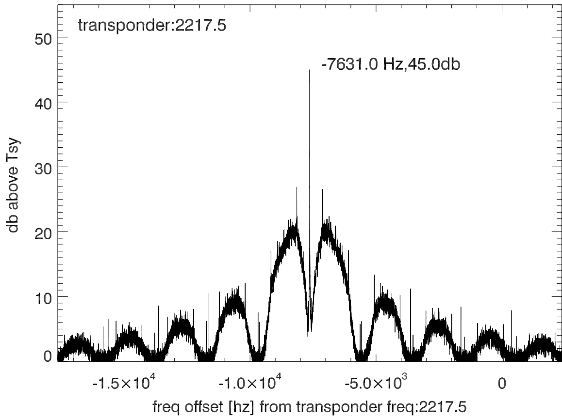
isee3 140606:203153 (UTC) spectra after doppler correction. PoIA
