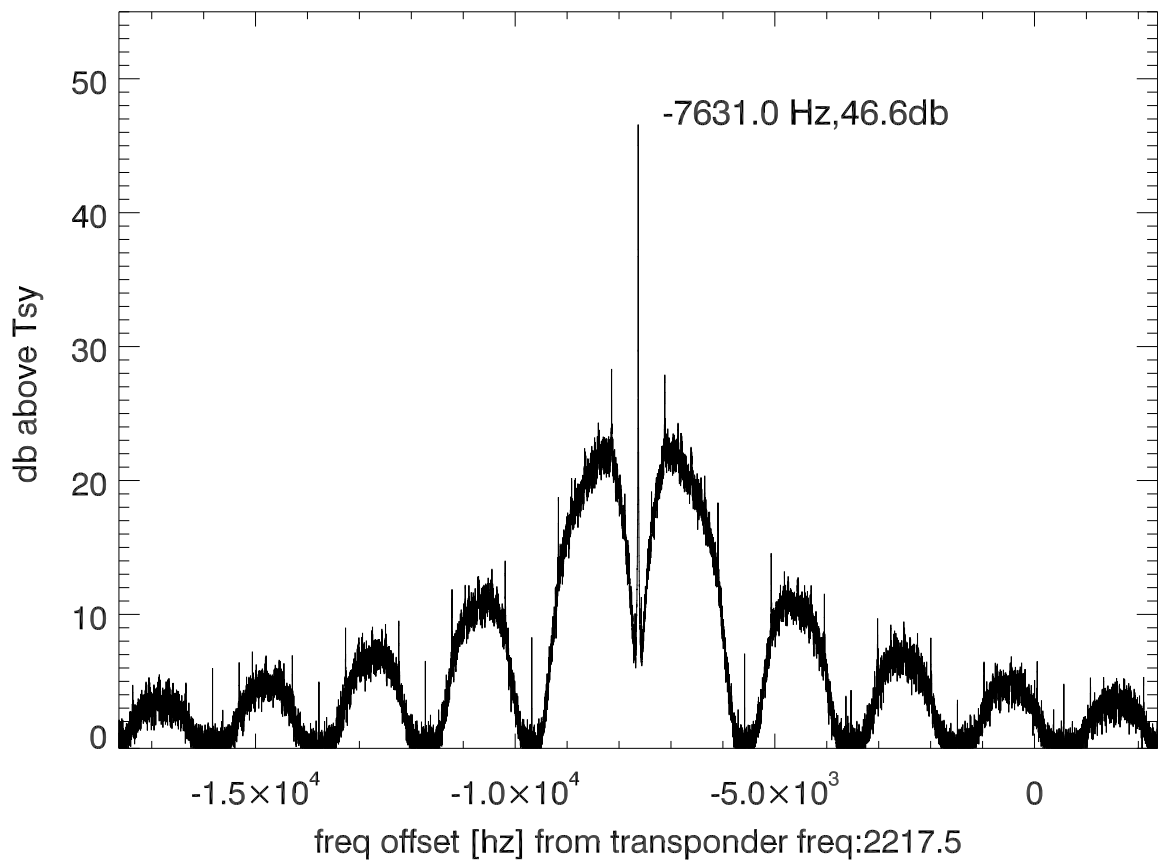
isee3 140606:203153 (UTC) spectra after doppler correction. PoIB
