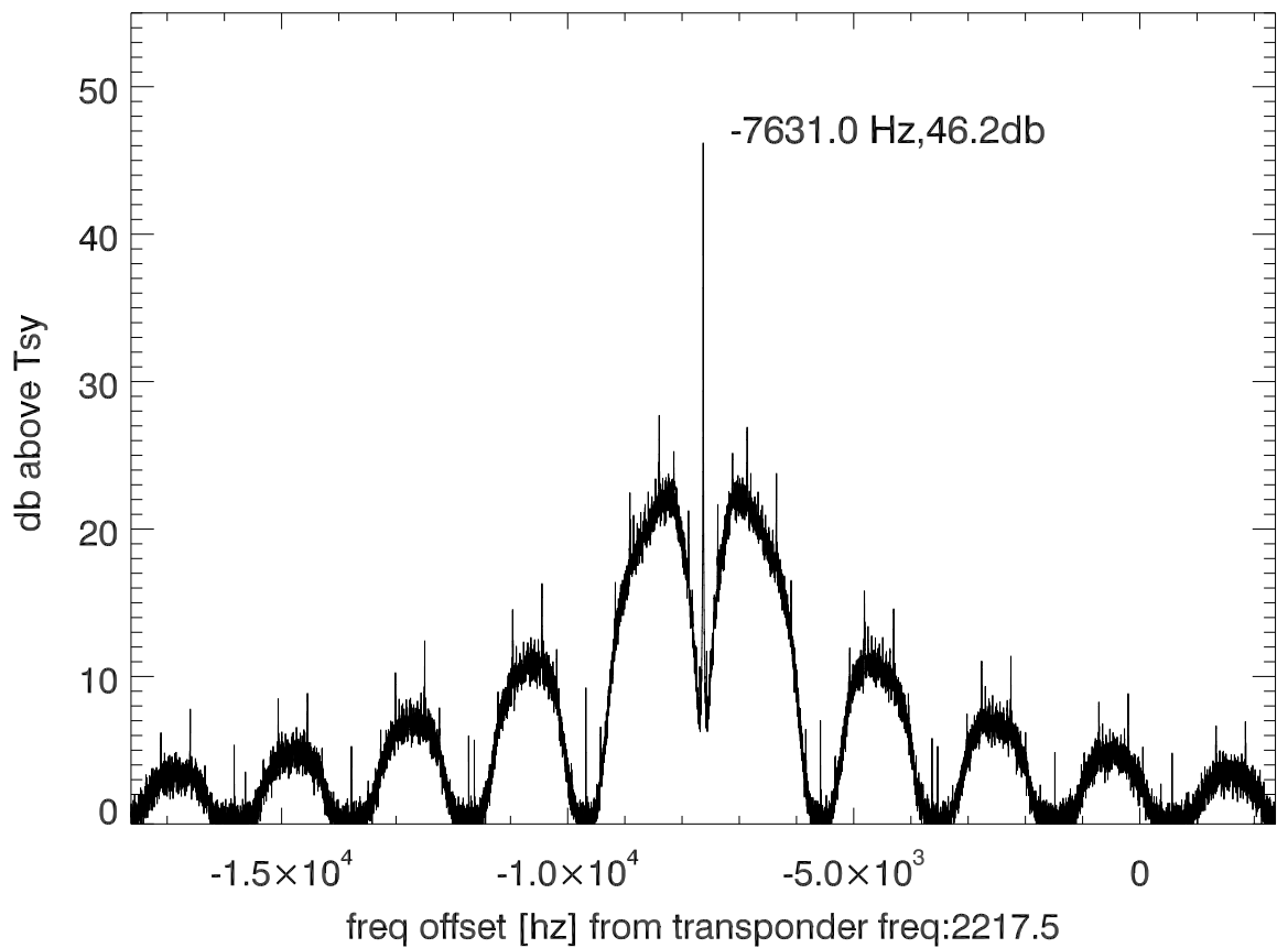
isee3 140606:202819 (UTC) spectra after doppler correction. PoIB
