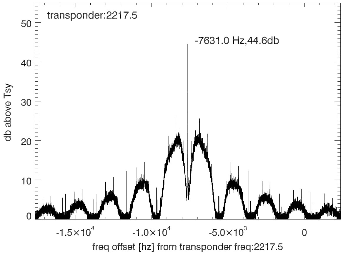
isee3 140606:202819 (UTC) spectra after doppler correction. PoIA
