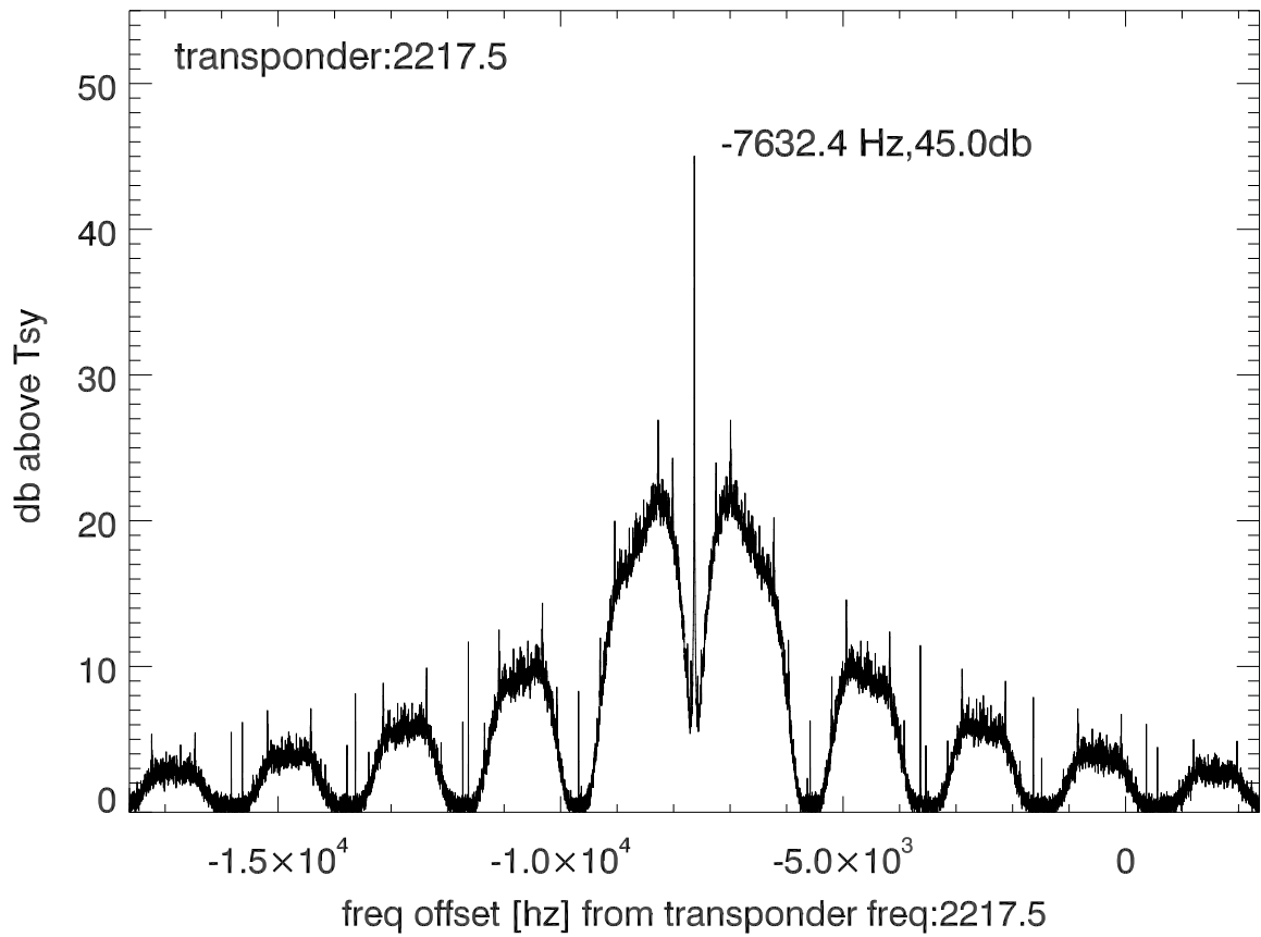
isee3 140606:192338 (UTC) spectra after doppler correction. PoIA
