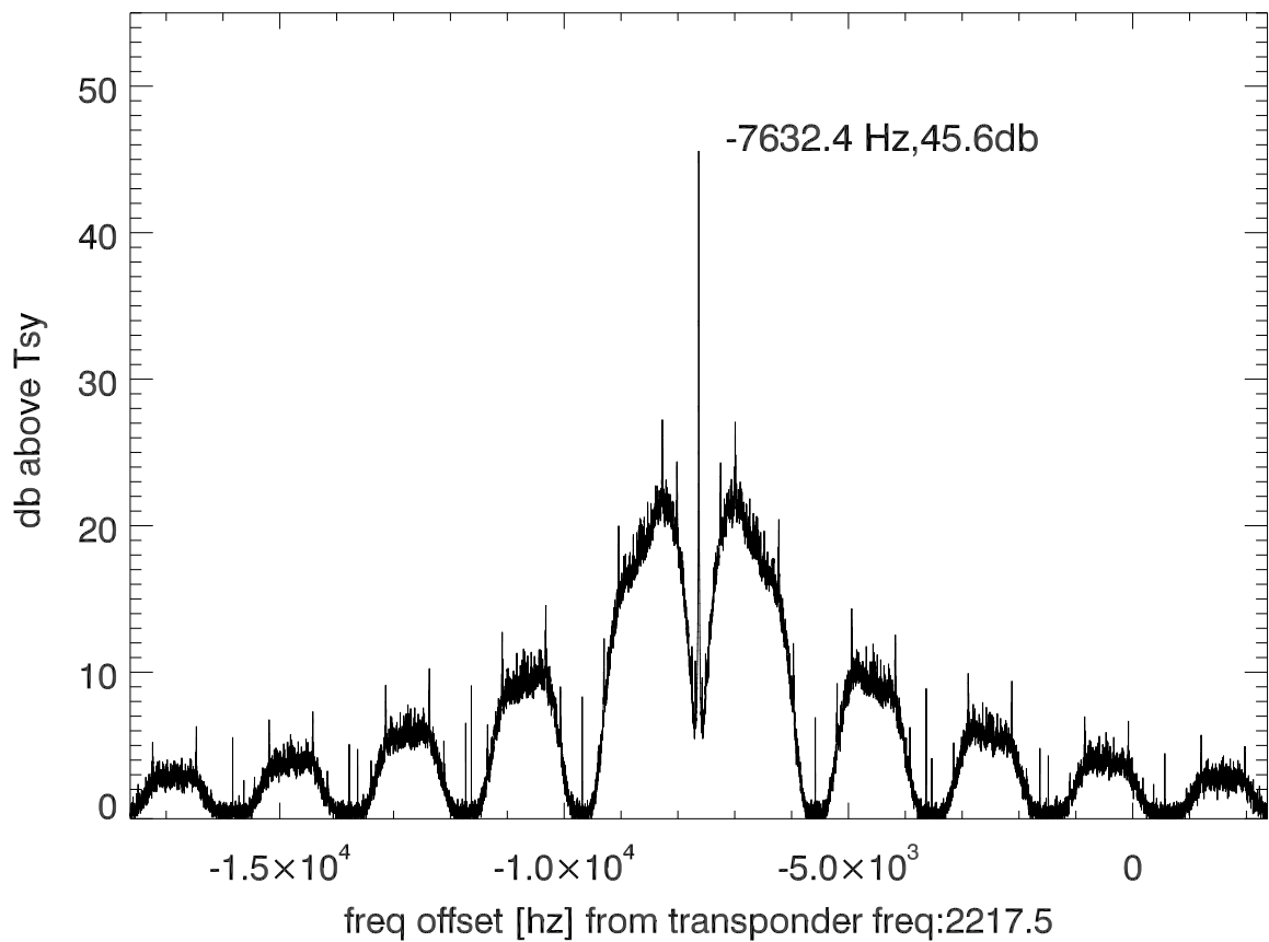
isee3 140606:192338 (UTC) spectra after doppler correction. PoIB
