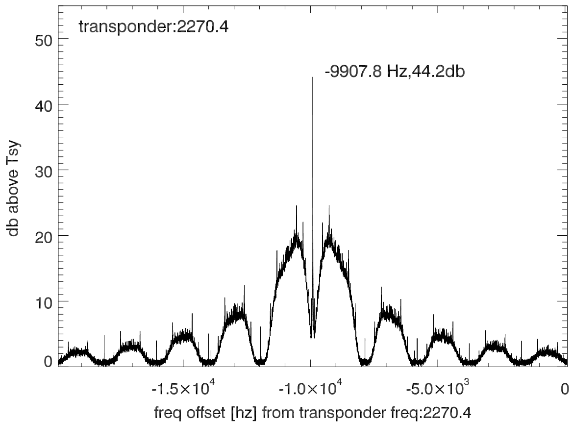
isee3 140603:204635 (UTC) spectra after doppler correction. PolA
