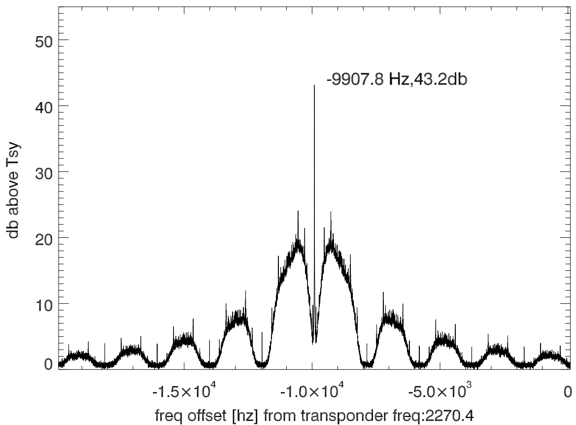
isee3 140603:204635 (UTC) spectra after doppler correction. PolB
