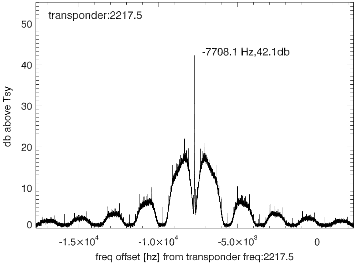
isee3 140603:204635 (UTC) spectra after doppler correction. PoIA
