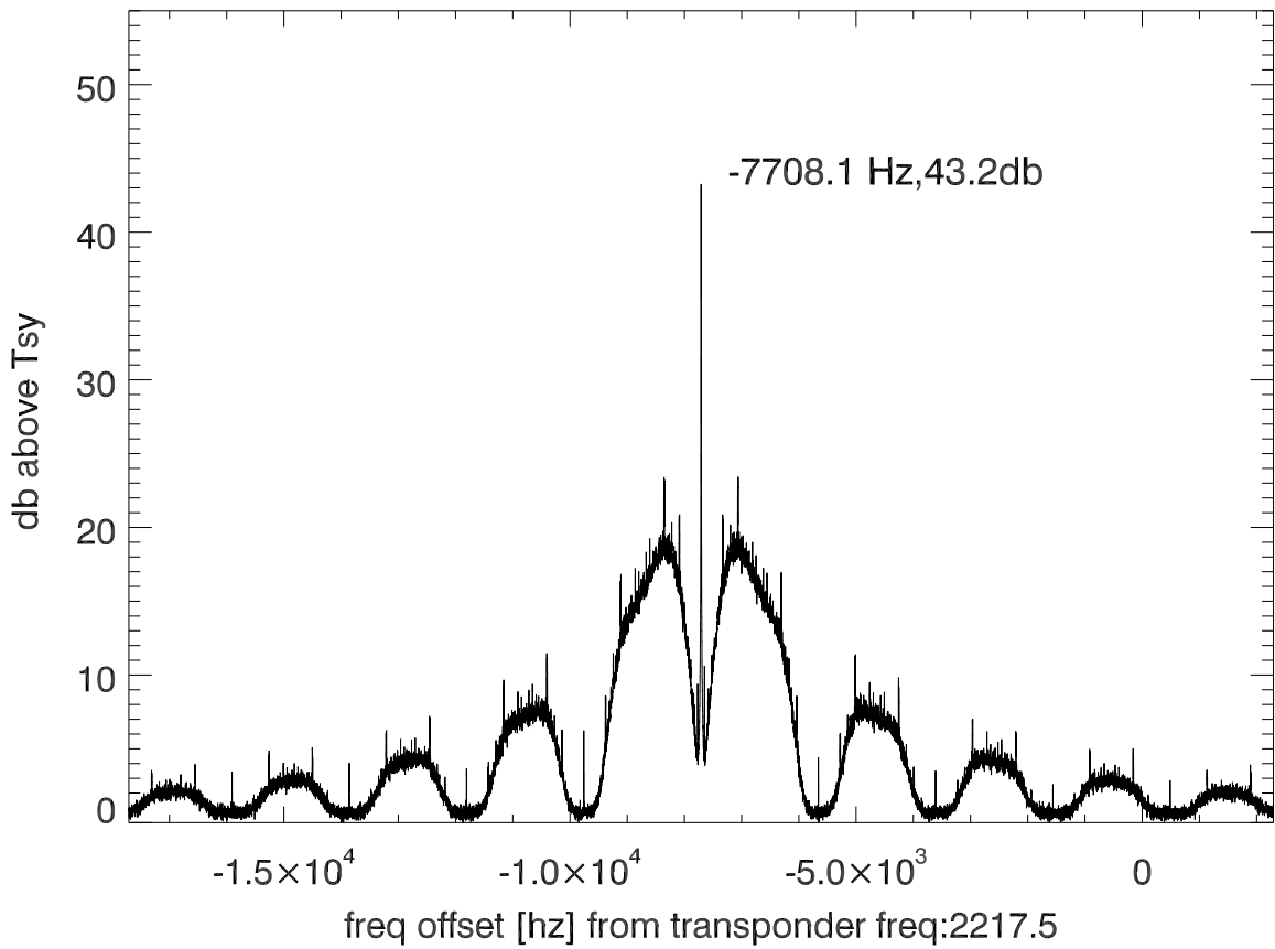
isee3 140603:204635 (UTC) spectra after doppler correction. PoIB
