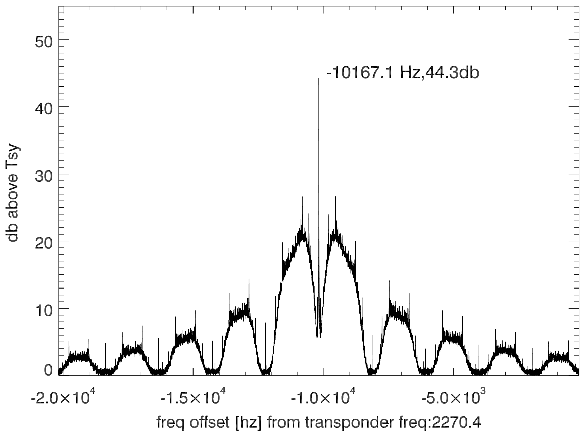
isee3 140530:205151 (UTC) spectra after doppler correction. PolB
