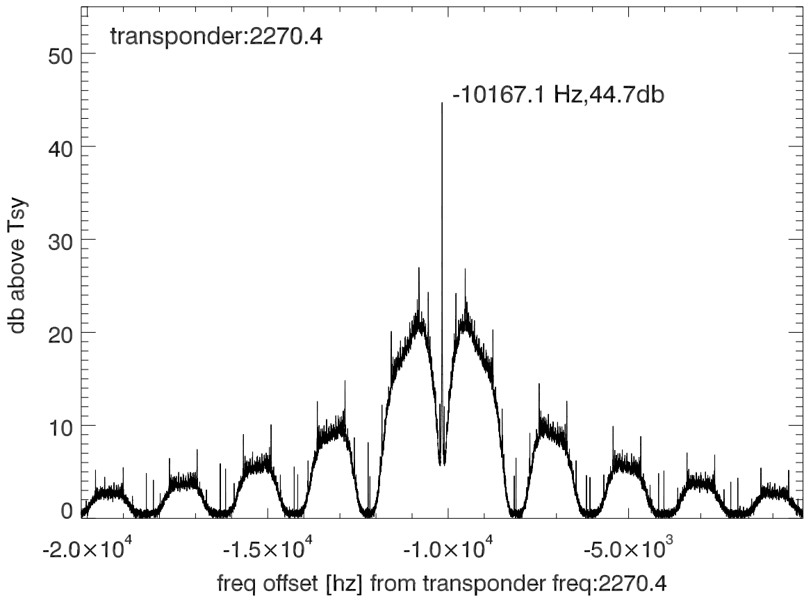
isee3 140530:205151 (UTC) spectra after doppler correction. PolA
