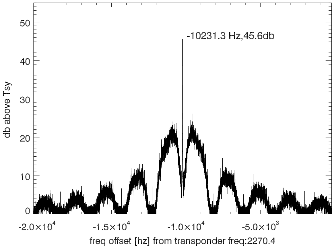
isee3 140529:203802 (UTC) spectra after doppler correction. PolB
