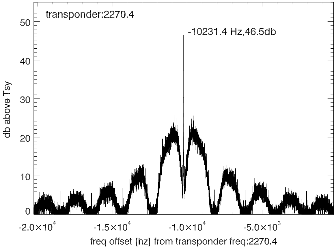
isee3 140529:203802 (UTC) spectra after doppler correction. PolA
