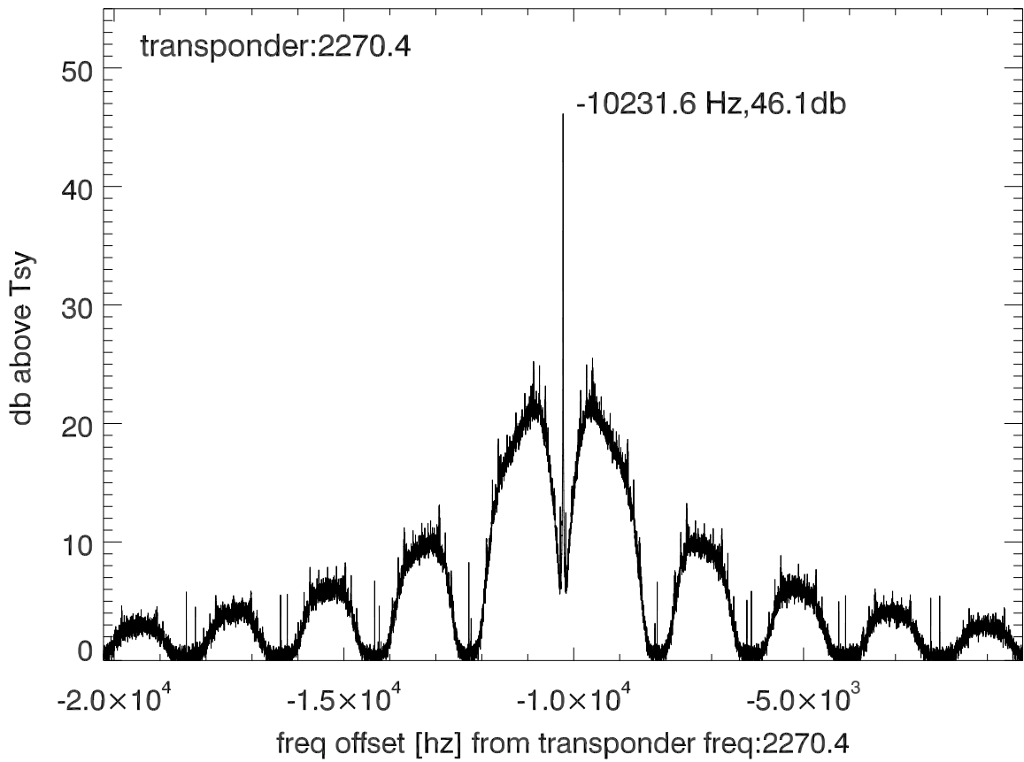
isee3 140529:202605 (UTC) spectra after doppler correction. PolA
