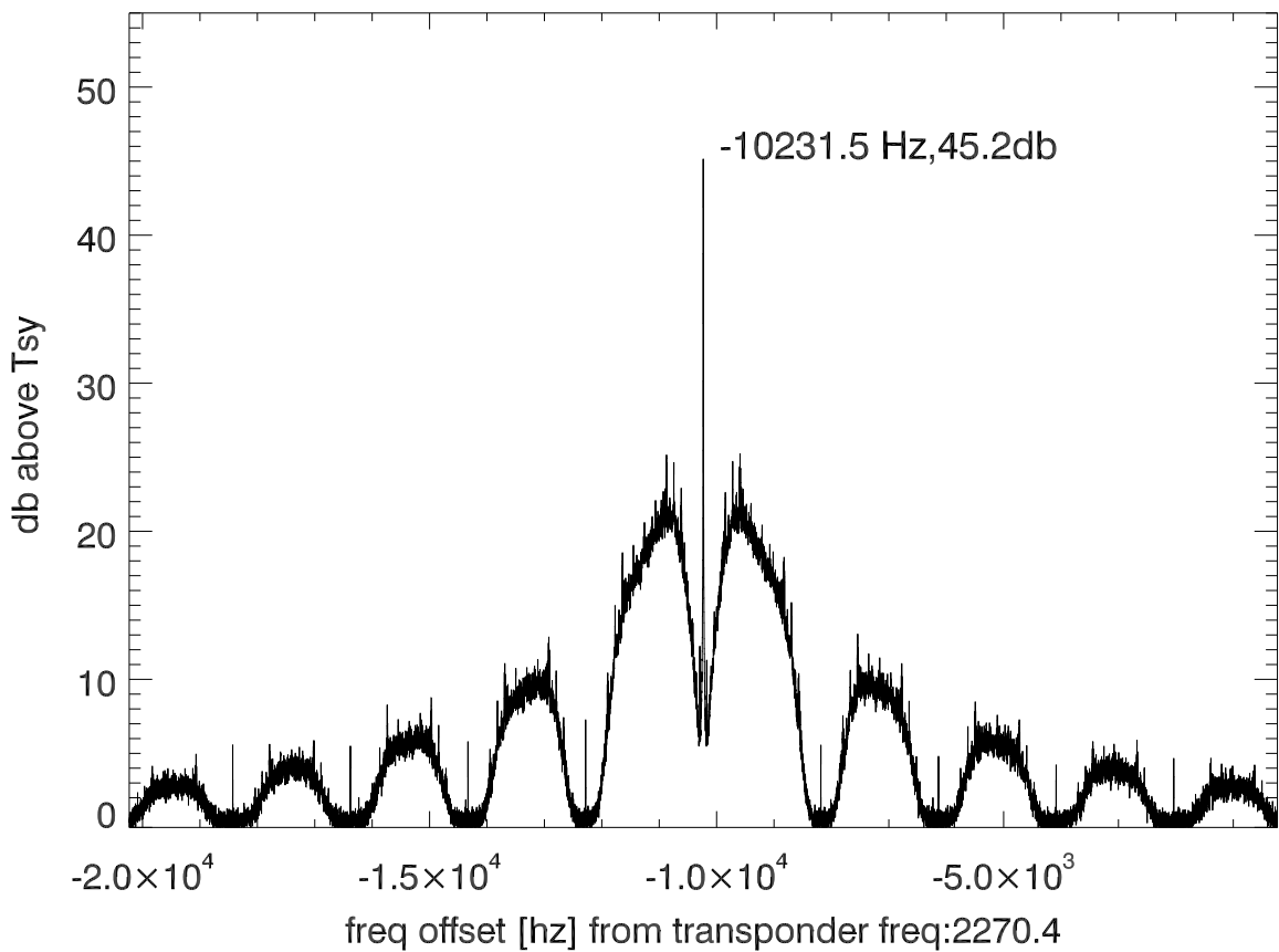
isee3 140529:202605 (UTC) spectra after doppler correction. PolB
