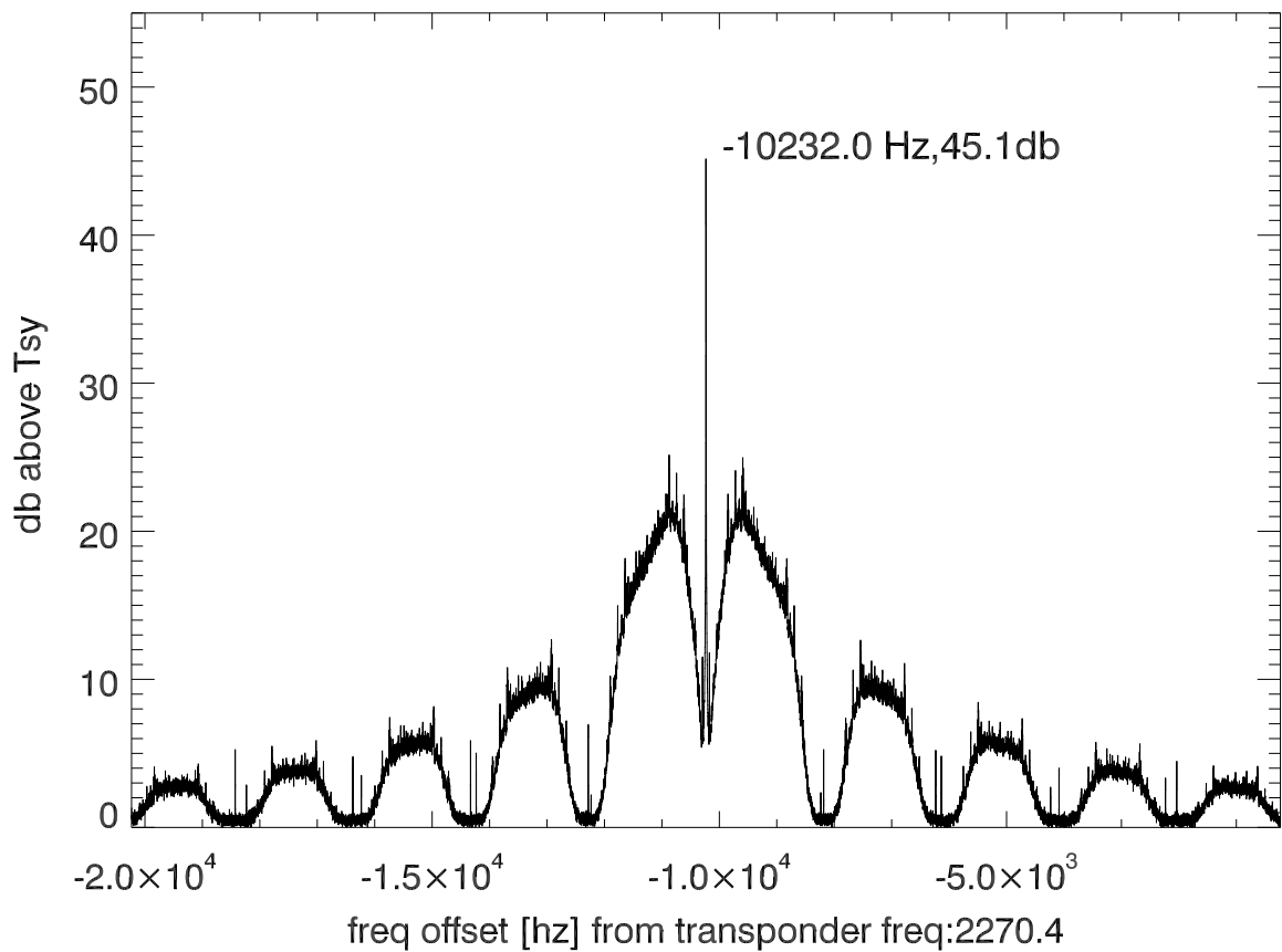
isee3 140529:201150 (UTC) spectra after doppler correction. PoIB
