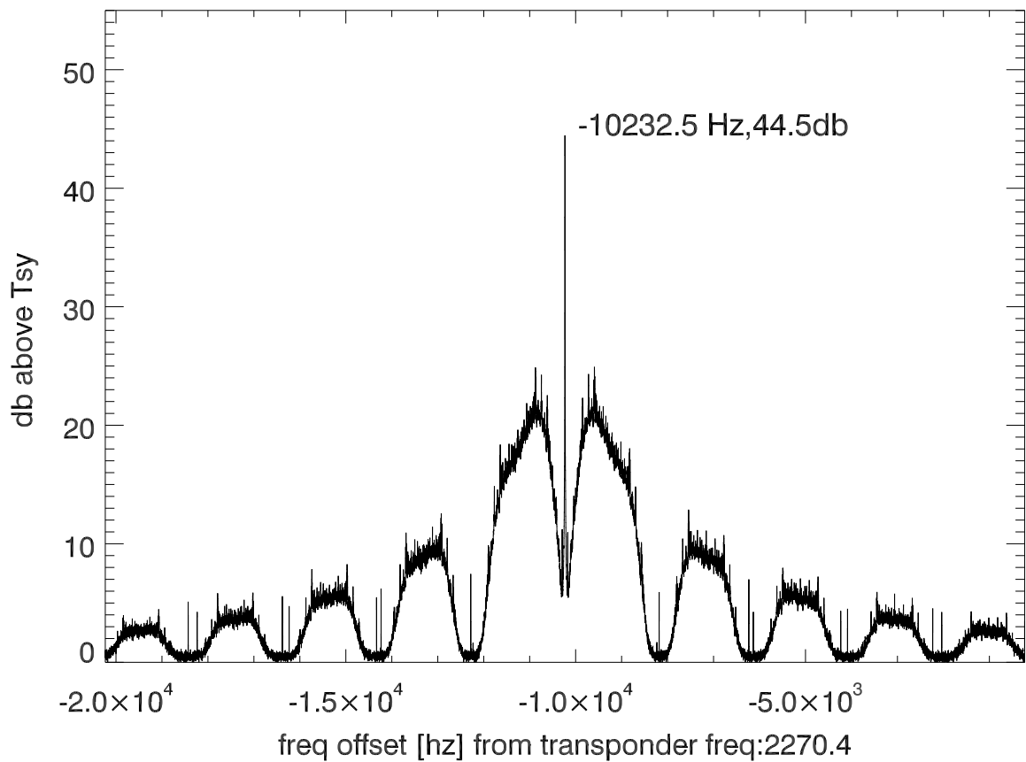
isee3 140529:200051 (UTC) spectra after doppler correction. PolB
