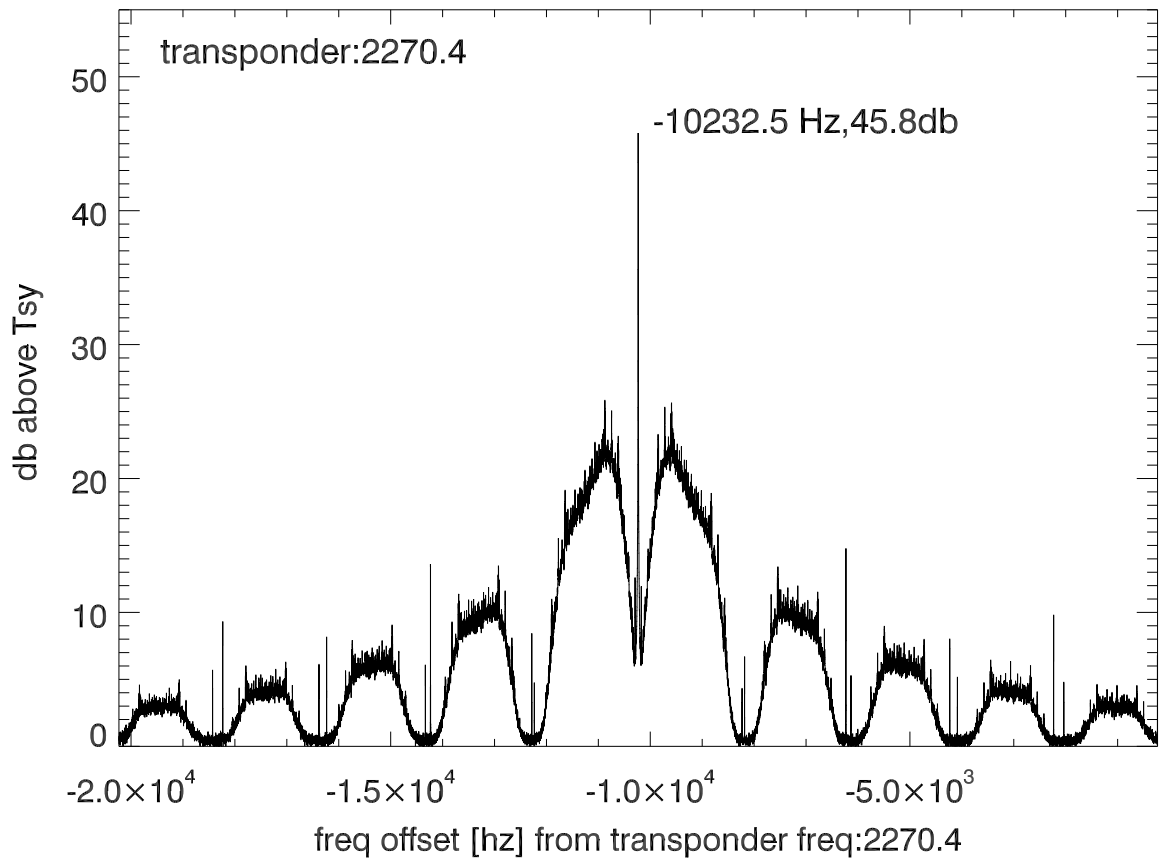
isee3 140529:200051 (UTC) spectra after doppler correction. PolA
