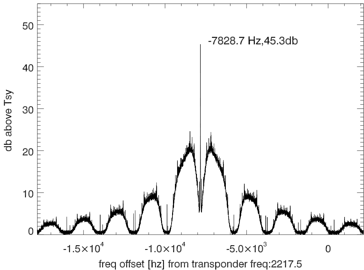
isee3 140529:200621 (UTC) spectra after doppler correction. PoIB
