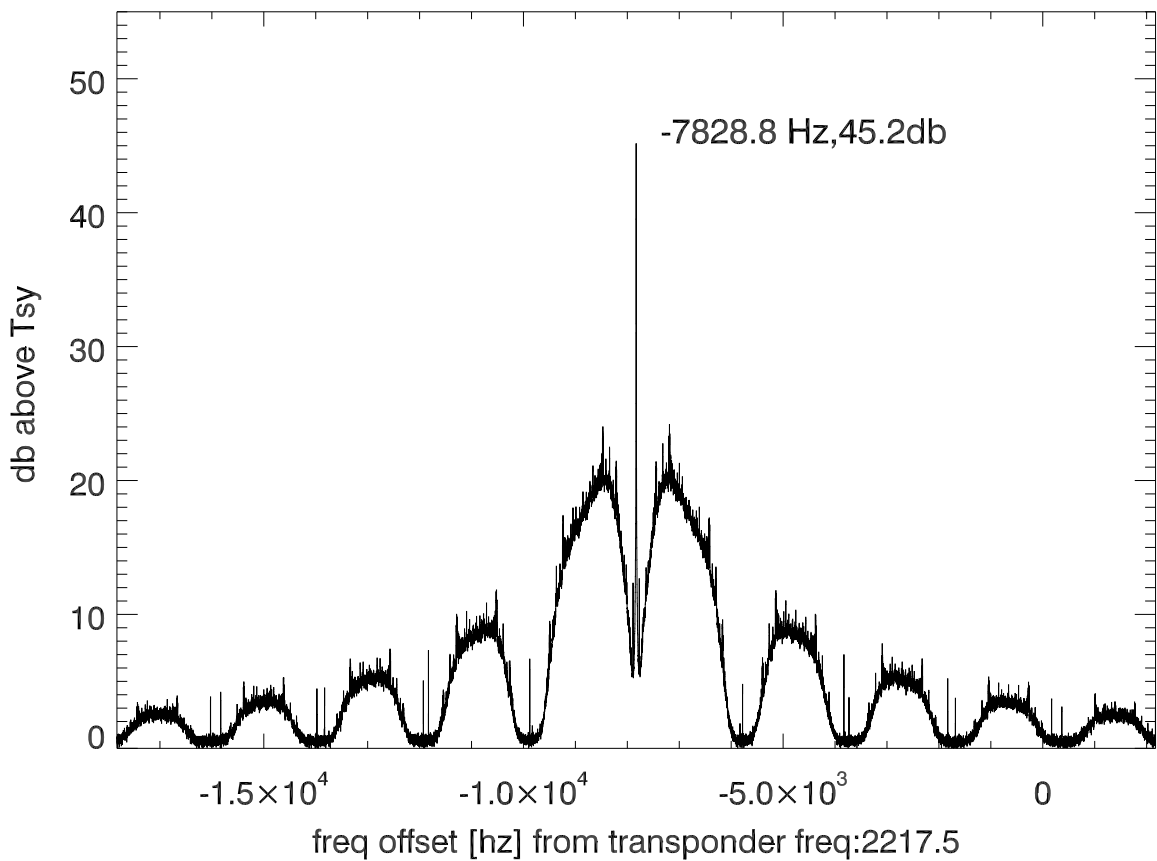
isee3 140529:200051 (UTC) spectra after doppler correction. PoIB
