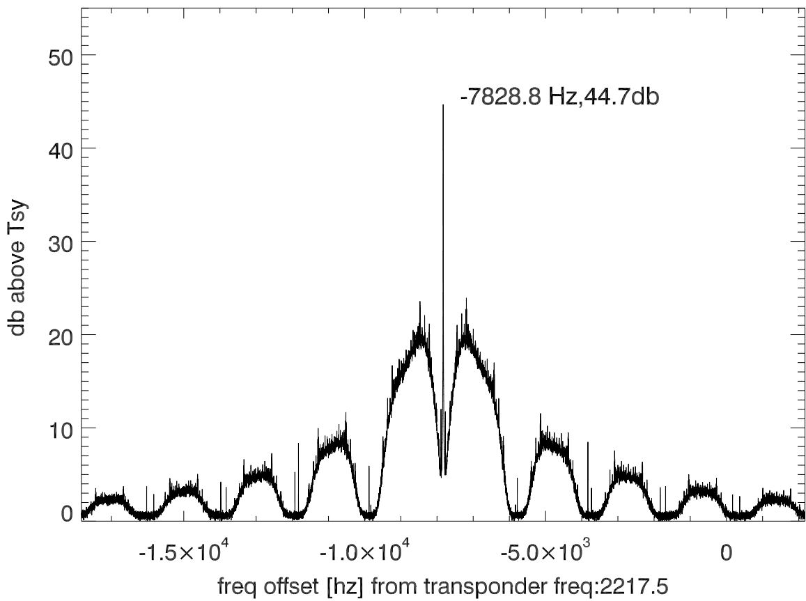
isee3 140529:195400 (UTC) spectra after doppler correction. PoIB
