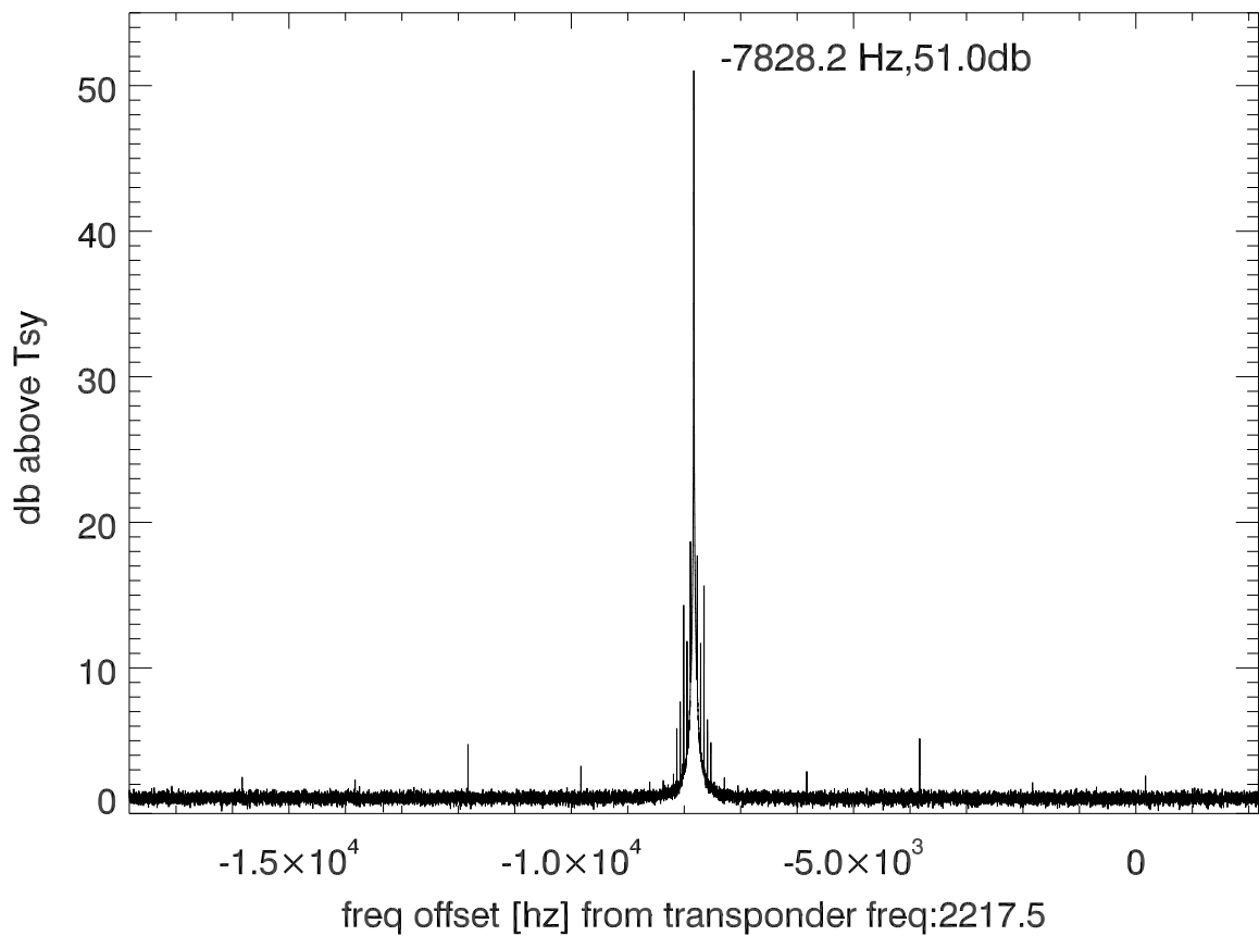
isee3 140528:205750 (UTC) spectra after doppler correction. PolB
