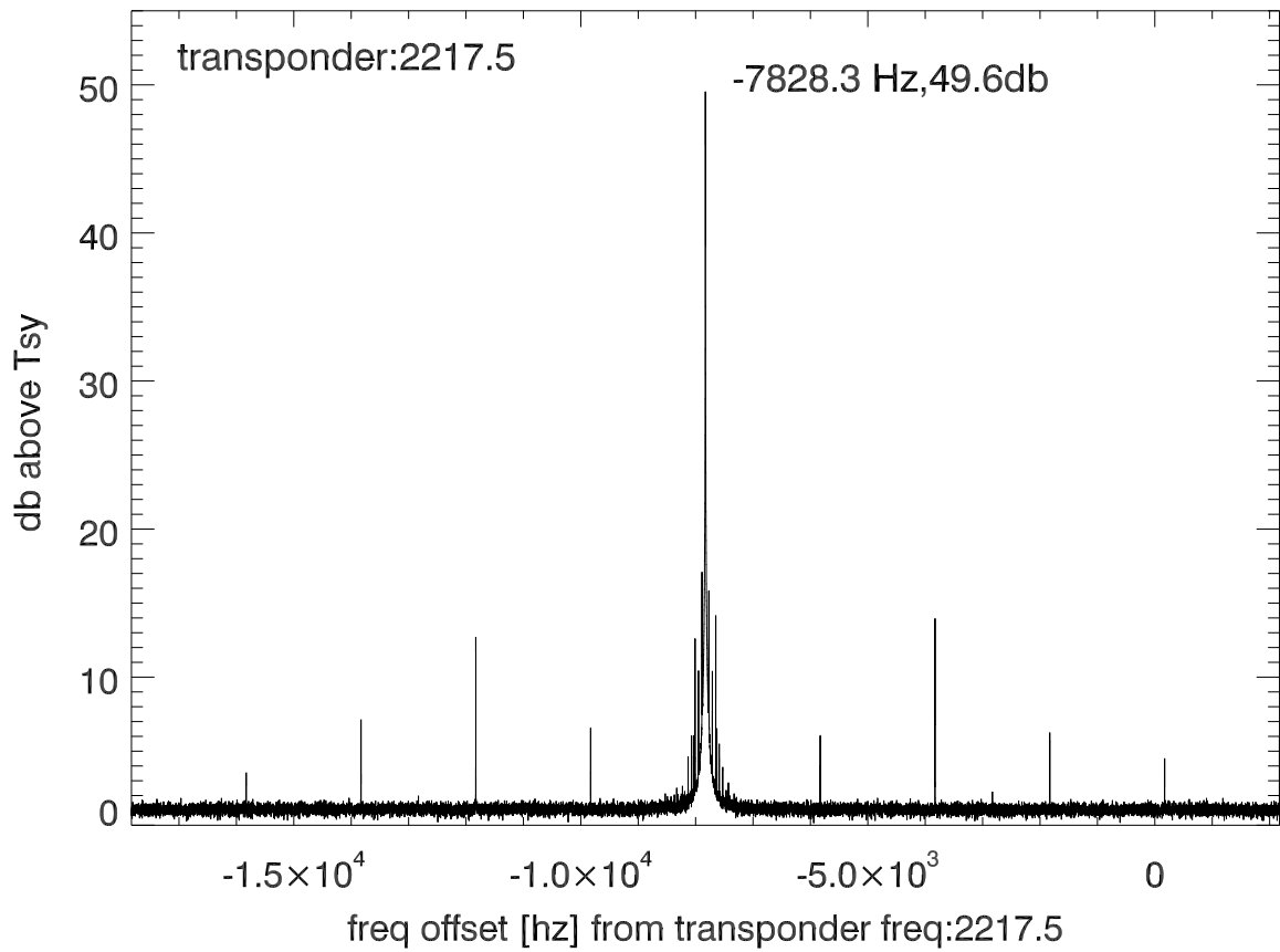
isee3 140528:205750 (UTC) spectra after doppler correction. PolA
