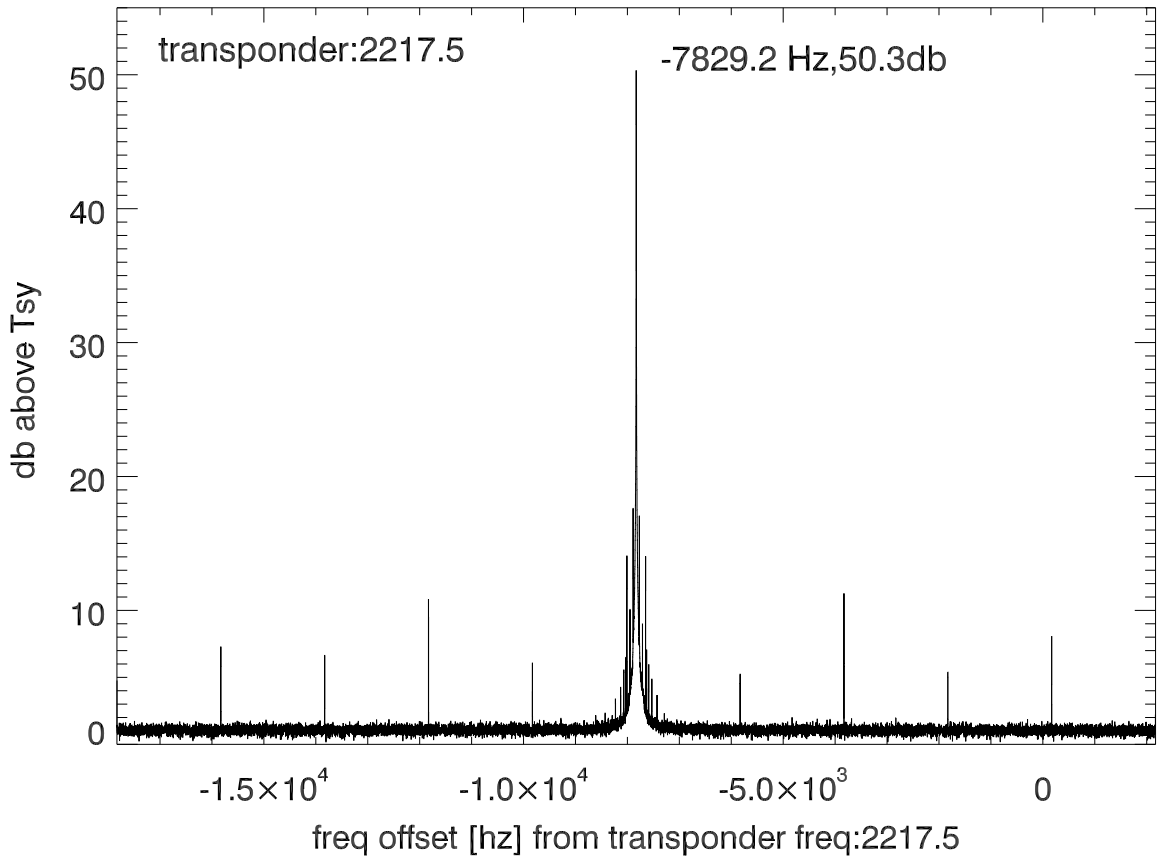
isee3 140528:204151 (UTC) spectra after doppler correction. PolA
