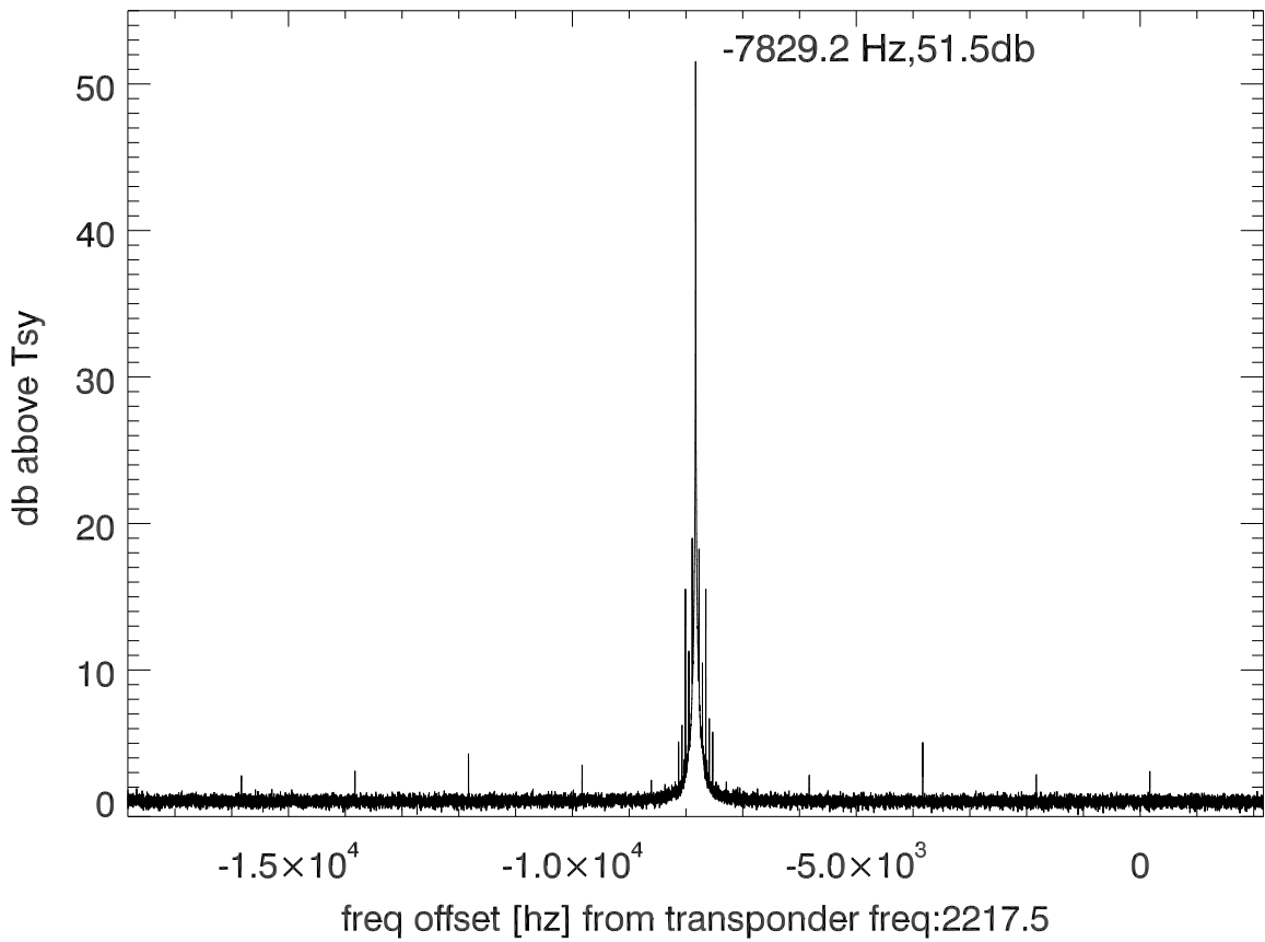
isee3 140528:204151 (UTC) spectra after doppler correction. PolB
