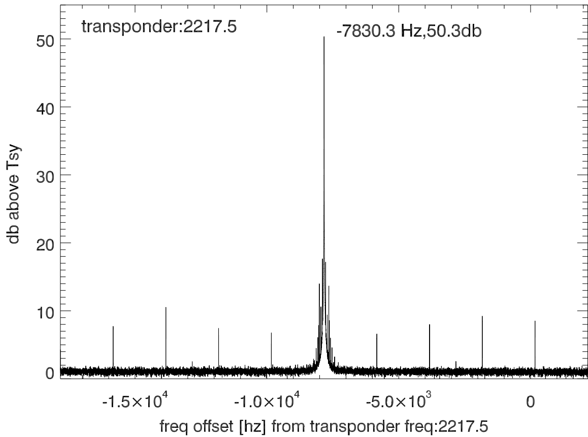
isee3 140528:202714 (UTC) spectra after doppler correction. PolA
