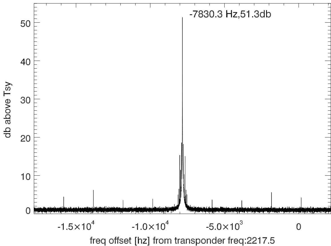
isee3 140528:202714 (UTC) spectra after doppler correction. PolB
