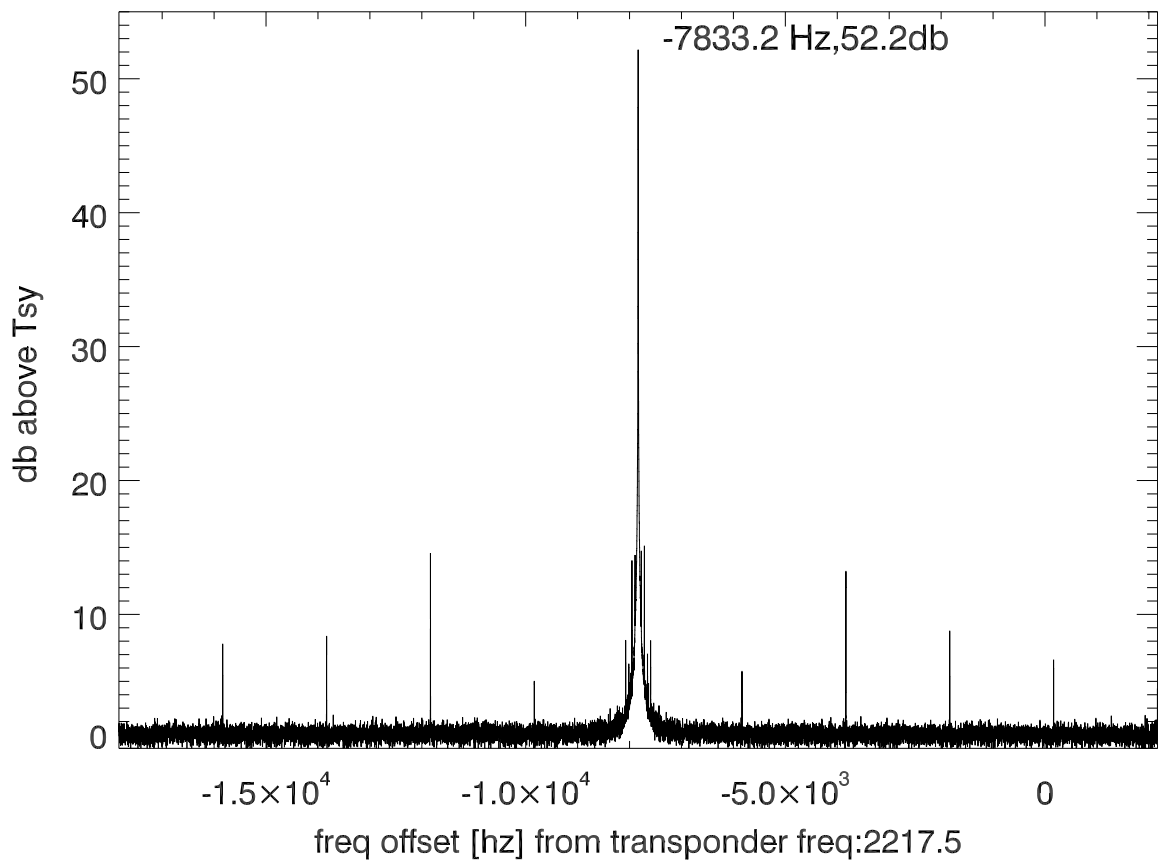
isee3 140528:192603 (UTC) spectra after doppler correction. PolB
