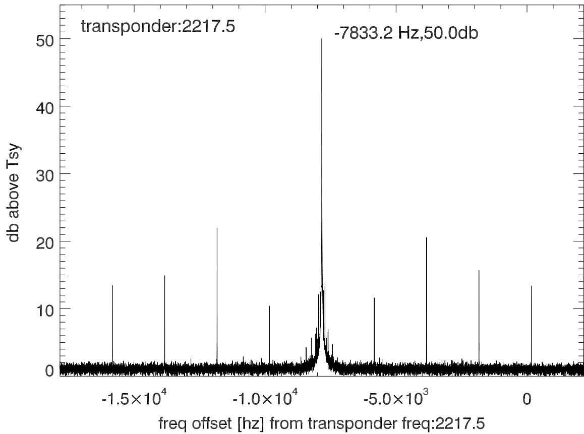
isee3 140528:192603 (UTC) spectra after doppler correction. PolA
