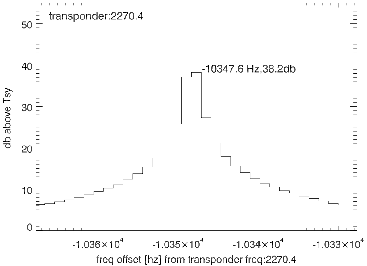
isee3 140527:203750 (UTC) spectra after doppler correction. PolA
