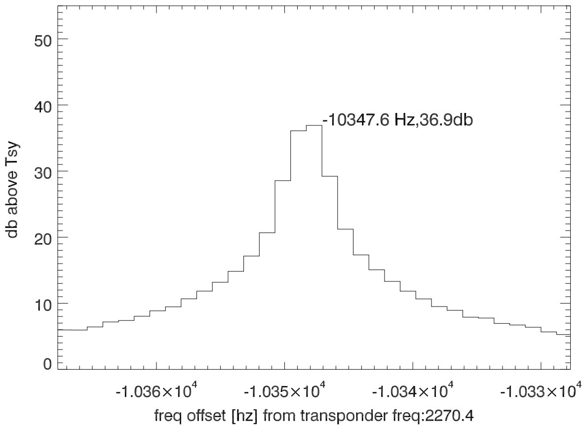
isee3 140527:203750 (UTC) spectra after doppler correction. PolB
