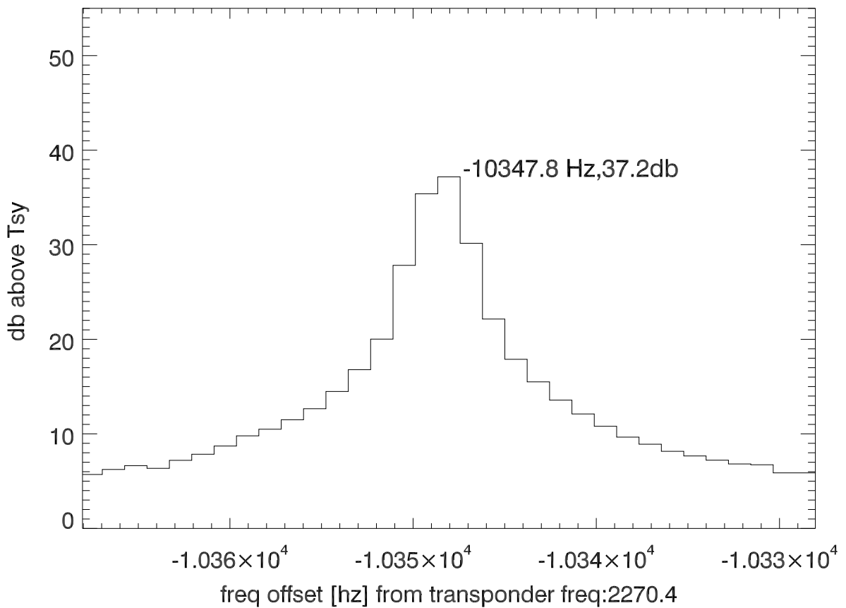
isee3 140527:203538 (UTC) spectra after doppler correction. PolB
