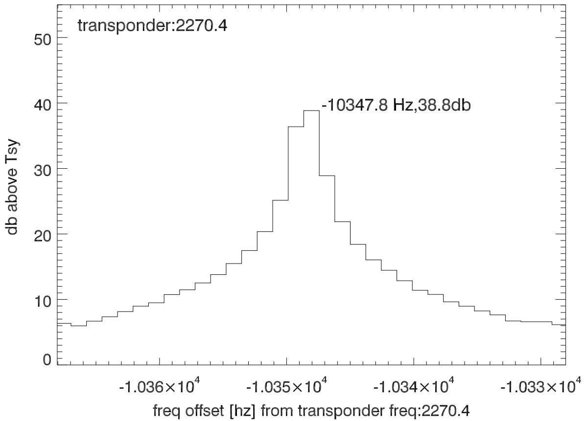
isee3 140527:203538 (UTC) spectra after doppler correction. PolA
