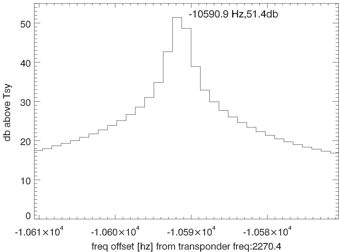
isee3 140523:192045 (UTC) spectra after doppler correction. PolB
