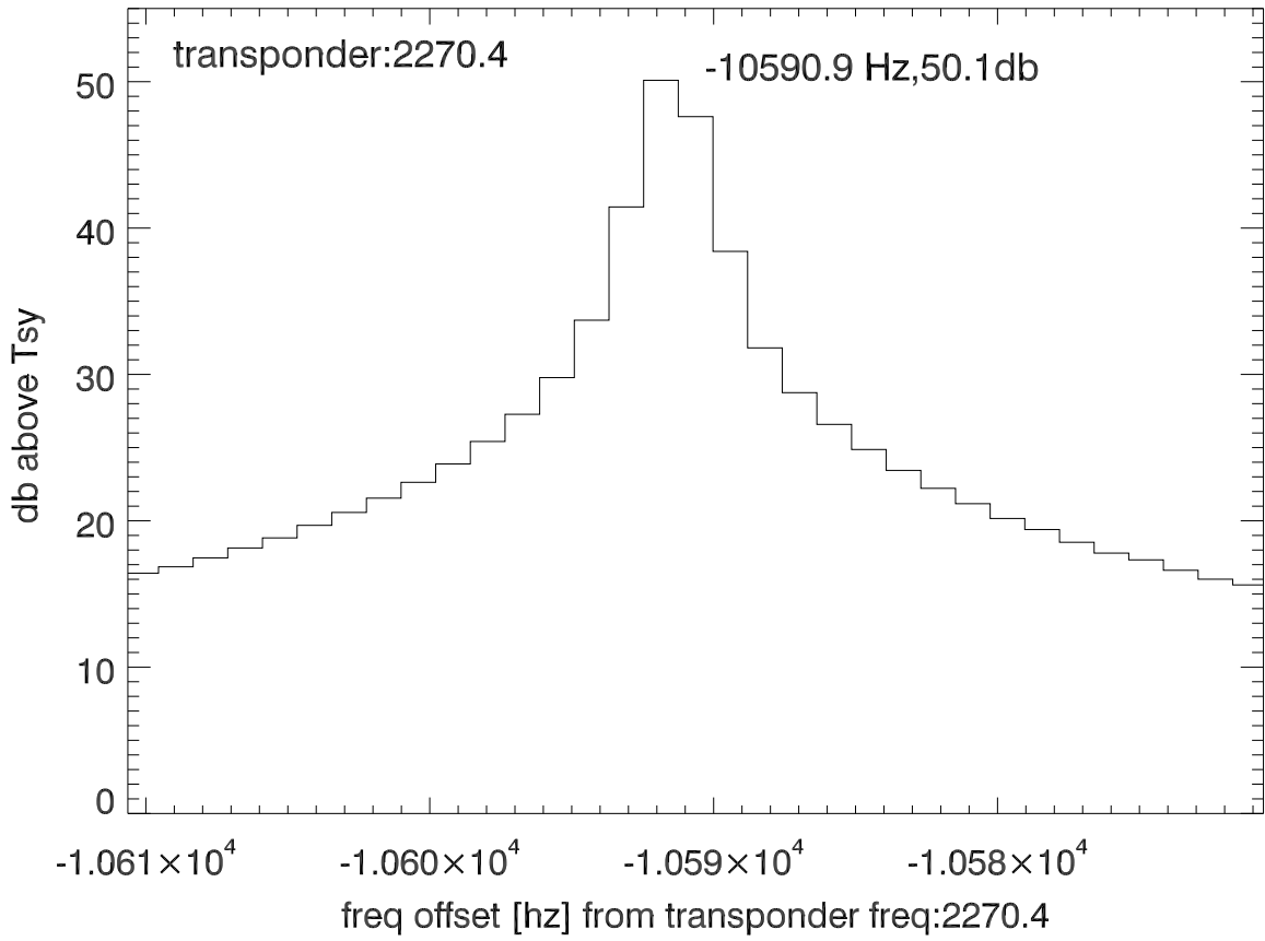
isee3 140523:192045 (UTC) spectra after doppler correction. PolA
