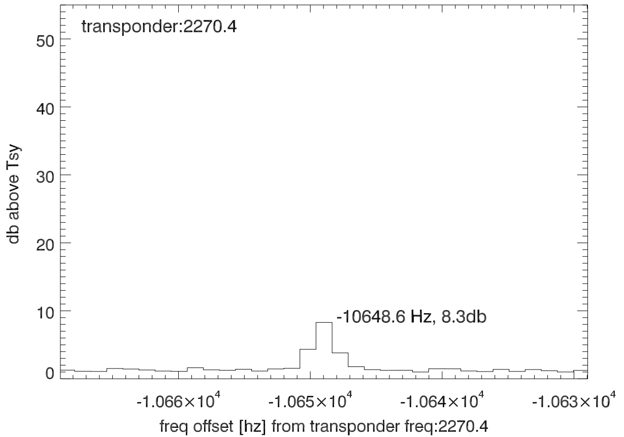
isee3 140522:201134 (UTC) spectra after doppler correction. PolA
