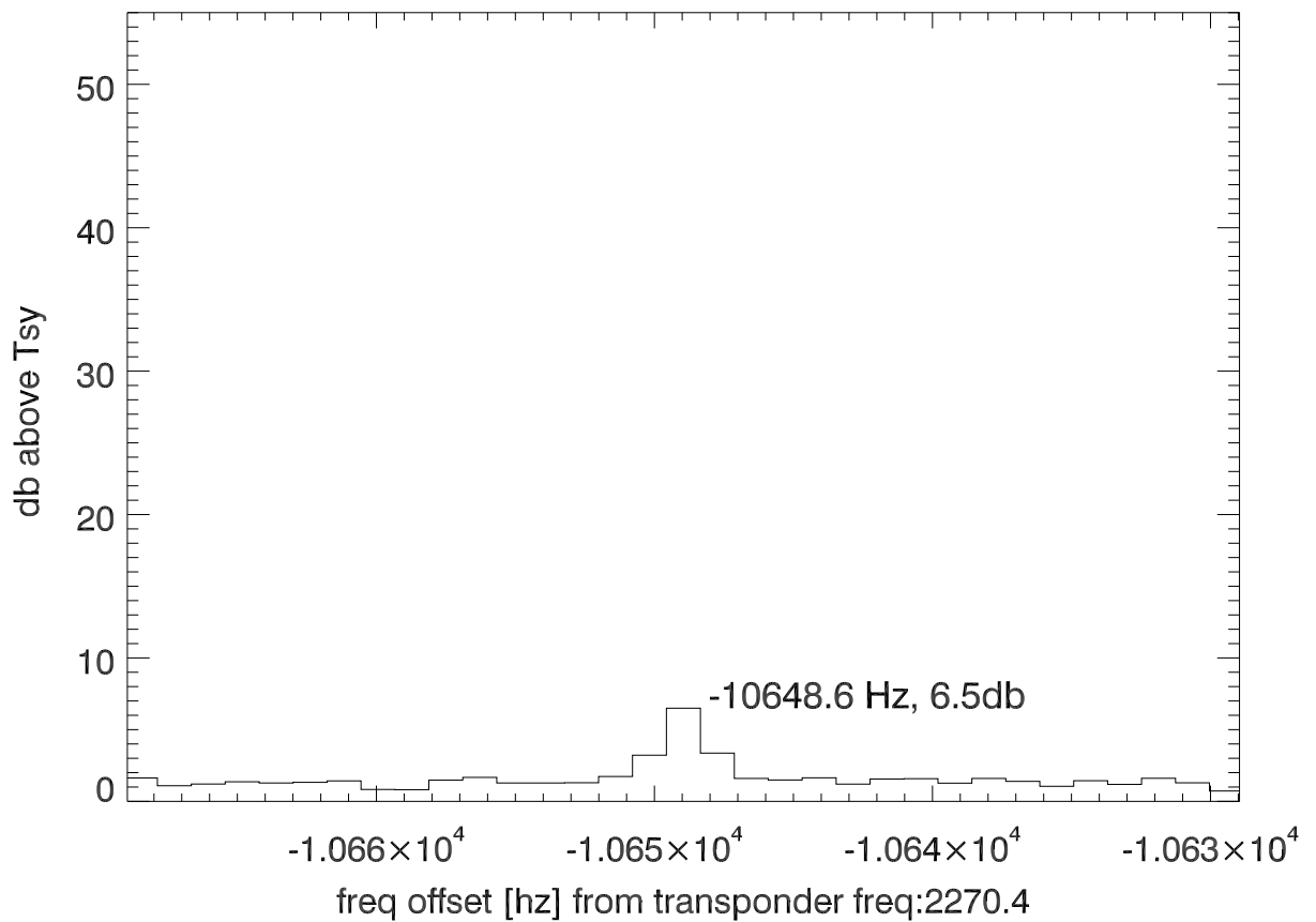
isee3 140522:201134 (UTC) spectra after doppler correction. PolB
