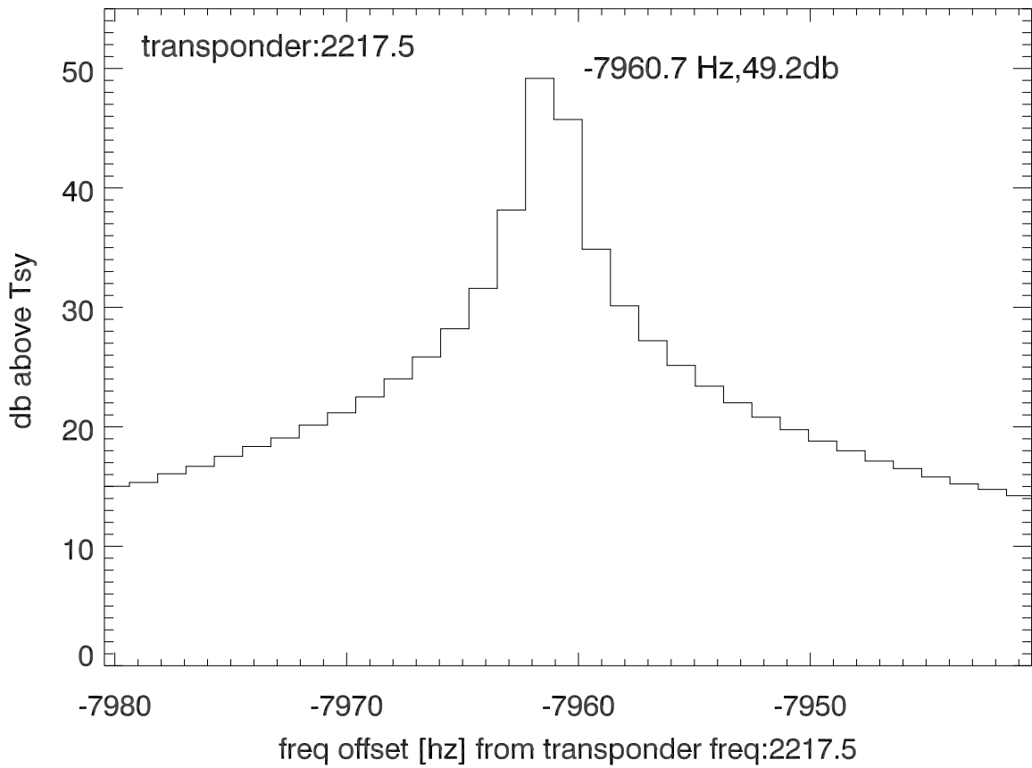
isee3 140522:204422 (UTC) spectra after doppler correction. PolA
