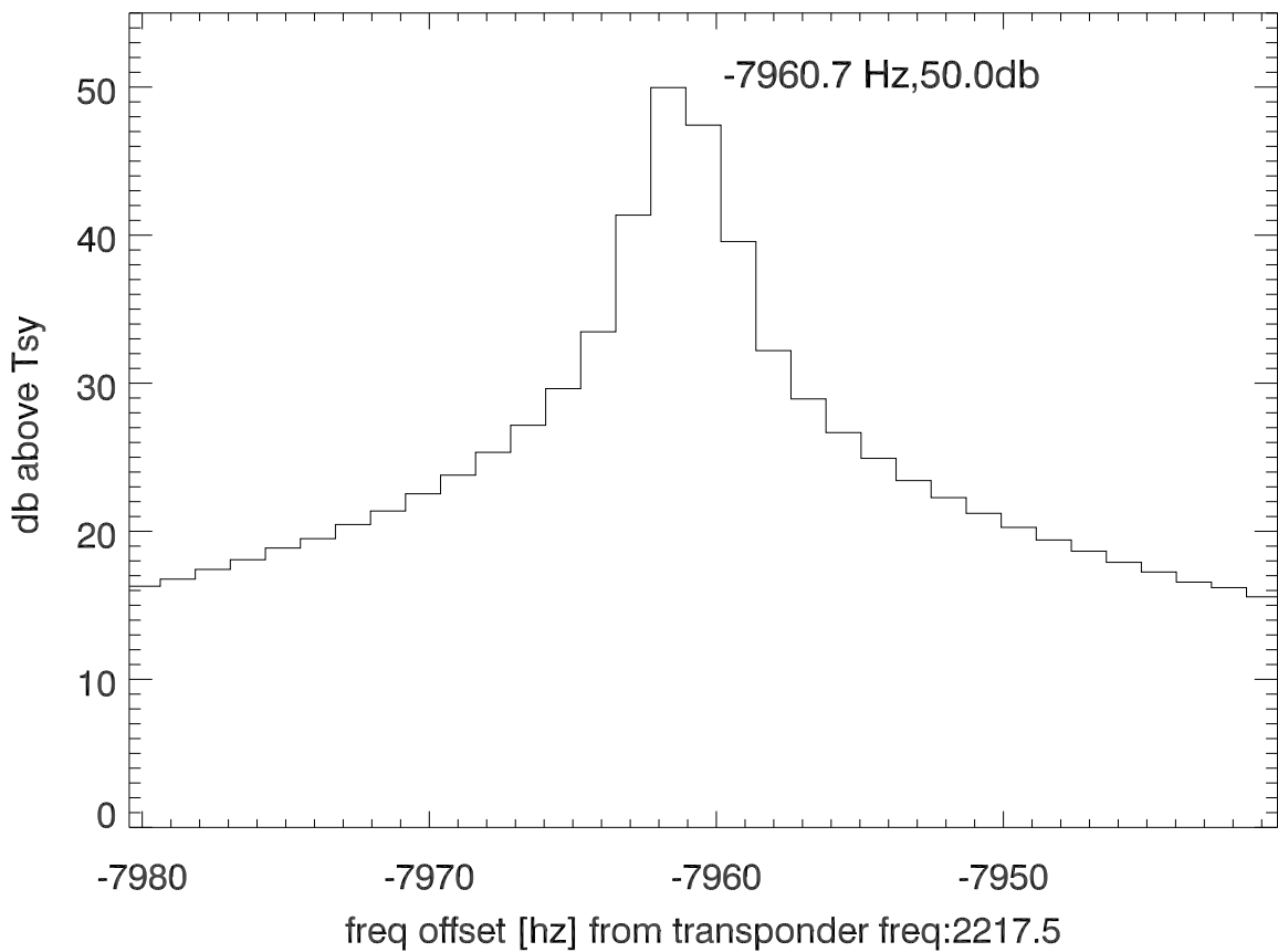
isee3 140522:204422 (UTC) spectra after doppler correction. PolB
