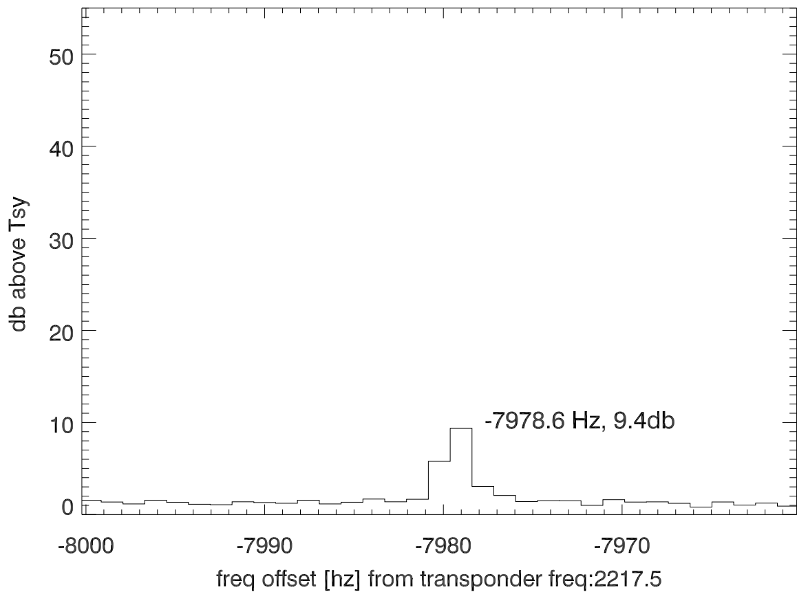
isee3 140521:200003 (UTC) spectra after doppler correction. PolB
