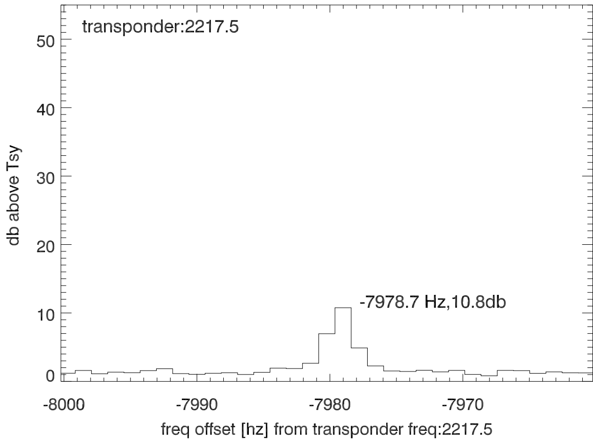
isee3 140521:200003 (UTC) spectra after doppler correction. PolA
