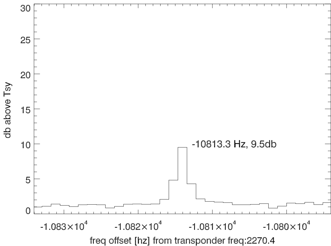
isee3 140519:185811 (UTC) spectra after doppler correction. PolB
