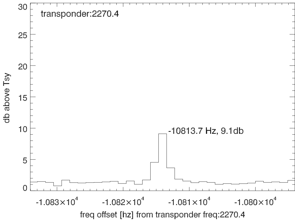
isee3 140519:185811 (UTC) spectra after doppler correction. PolA
