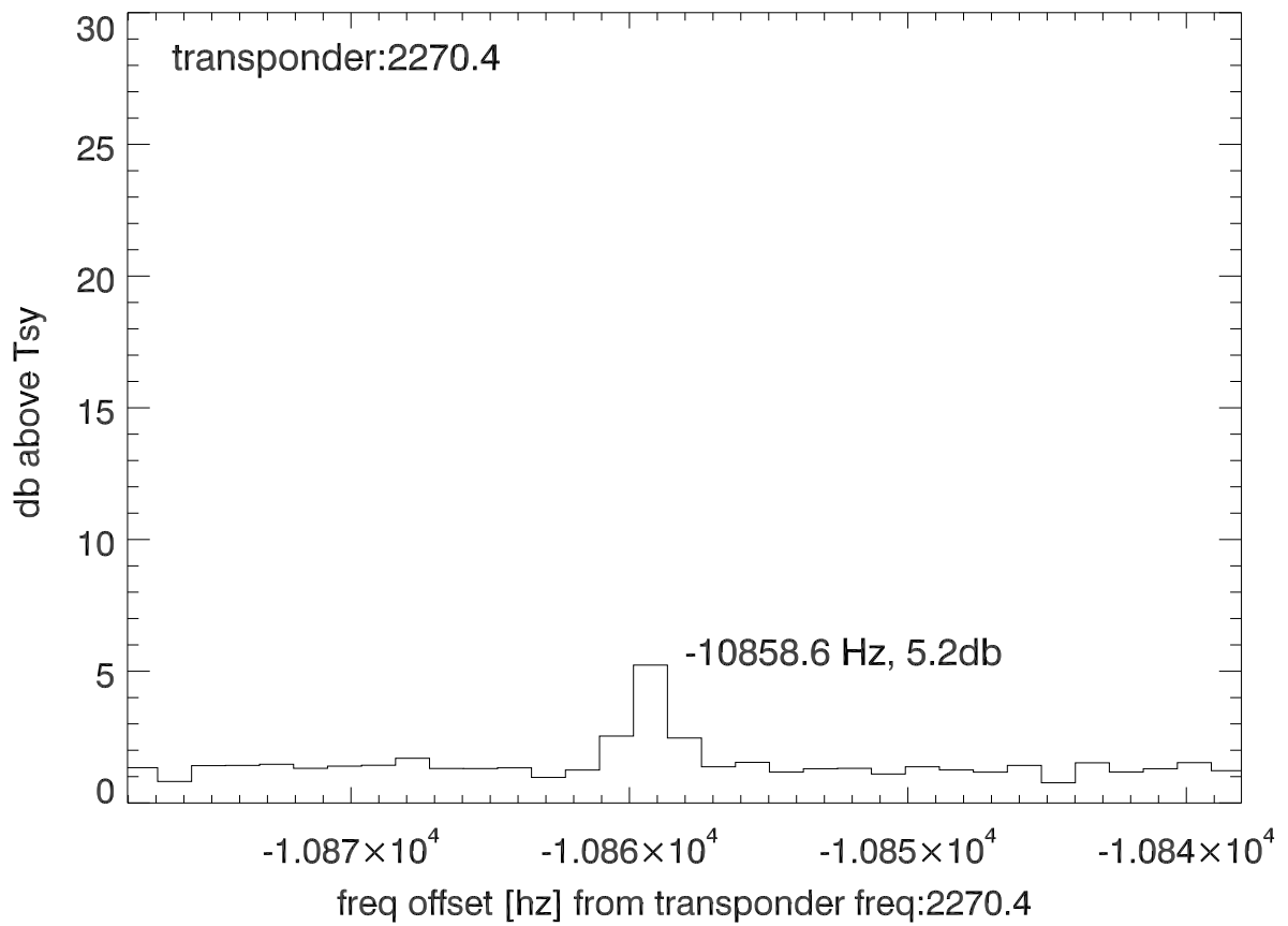
isee3 140518:210139 (UTC) spectra after doppler correction. PolA
