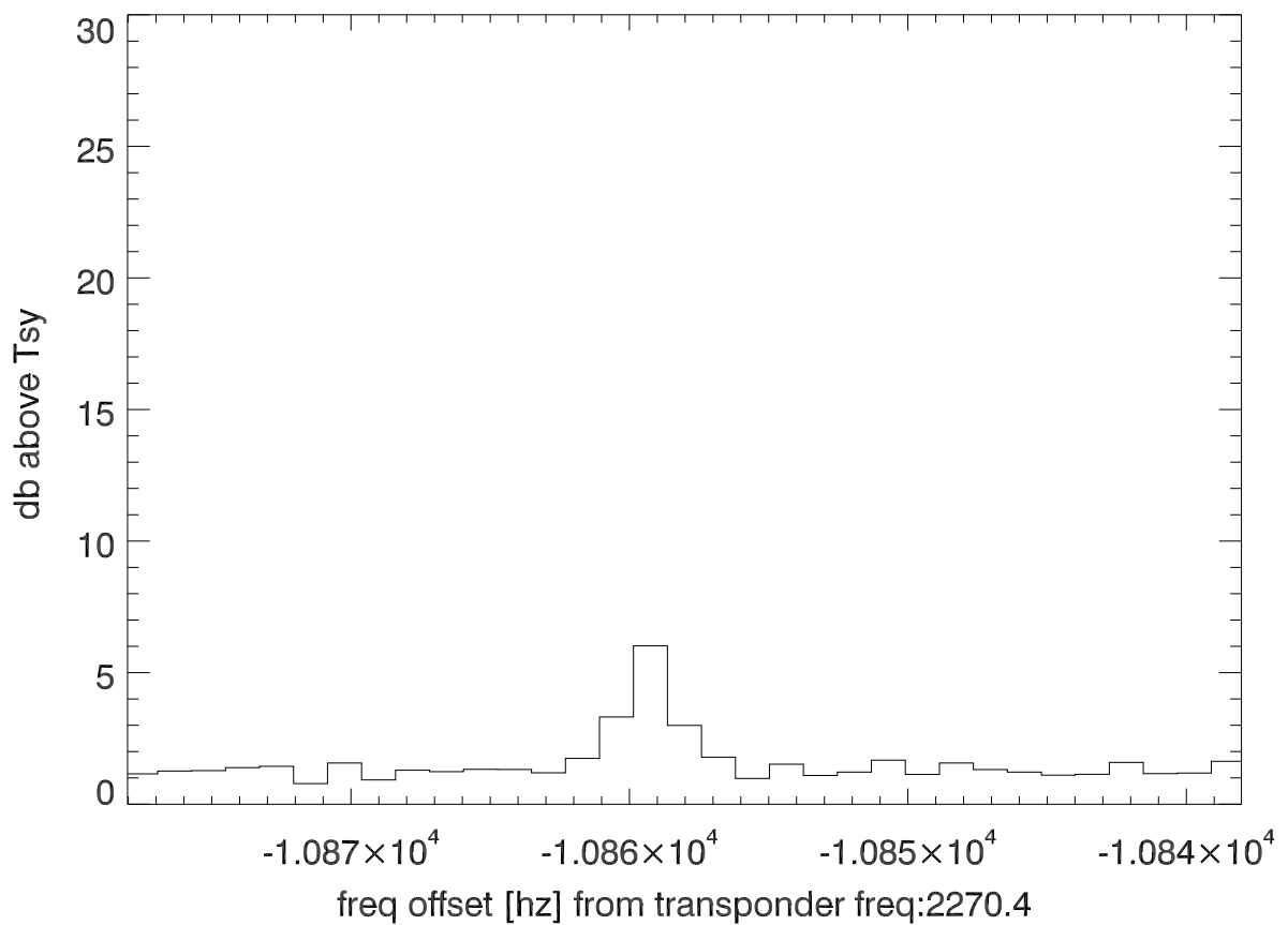
isee3 140518:210139 (UTC) spectra after doppler correction. PolB
