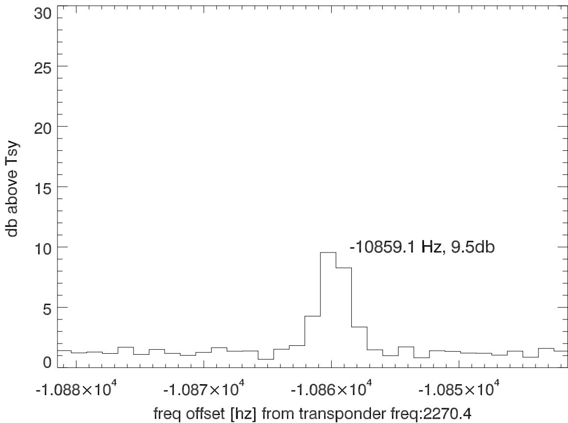
isee3 140518:205406 (UTC) spectra after doppler correction. PolB
