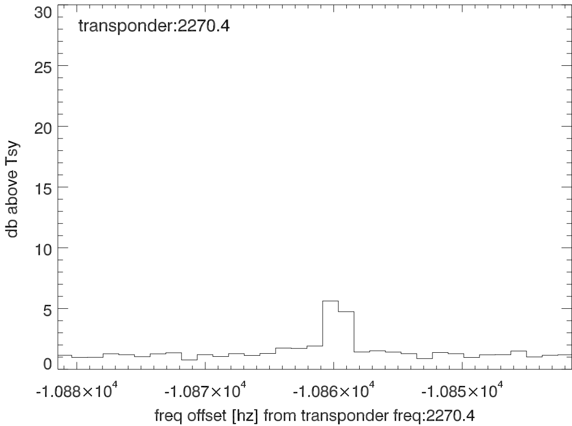
isee3 140518:205406 (UTC) spectra after doppler correction. PolA
