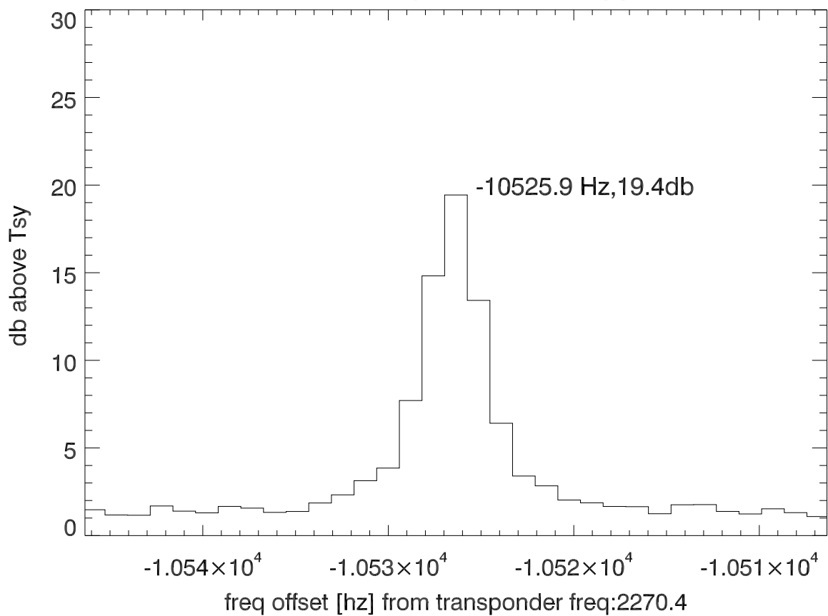
isee3 140414:205944 (UTC) spectra after doppler correction. PoIB
