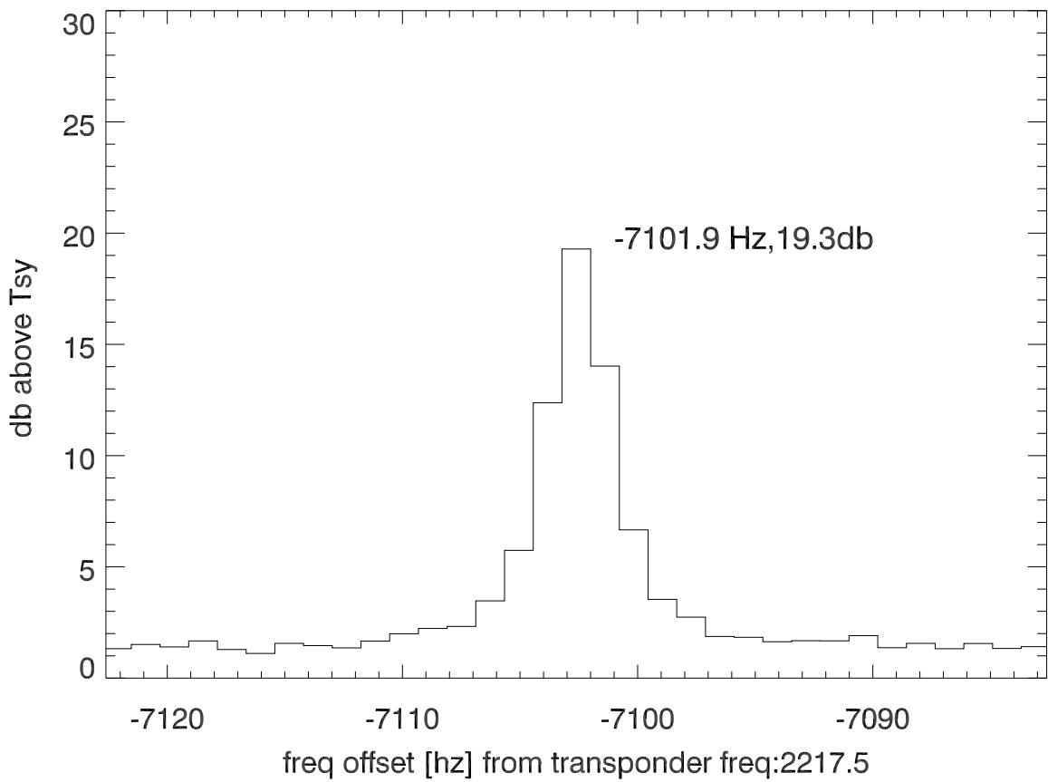
isee3 140414:205944 (UTC) spectra after doppler correction. PolB
