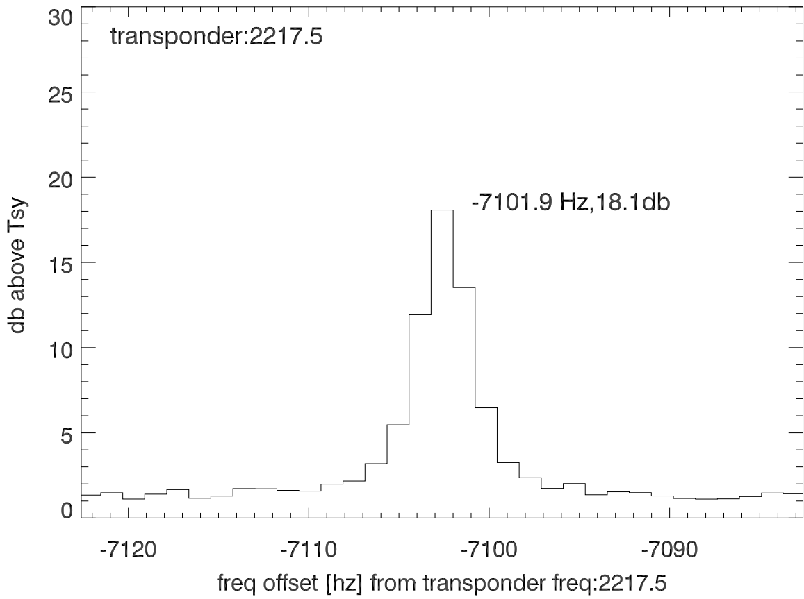
isee3 140414:205944 (UTC) spectra after doppler correction. PolA
