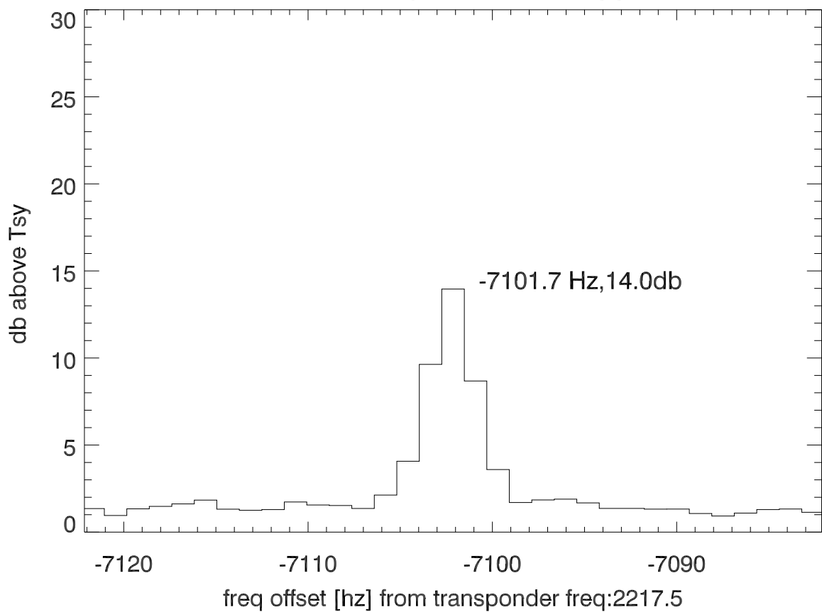
isee3 140414:200746 (UTC) spectra after doppler correction. PoIB
